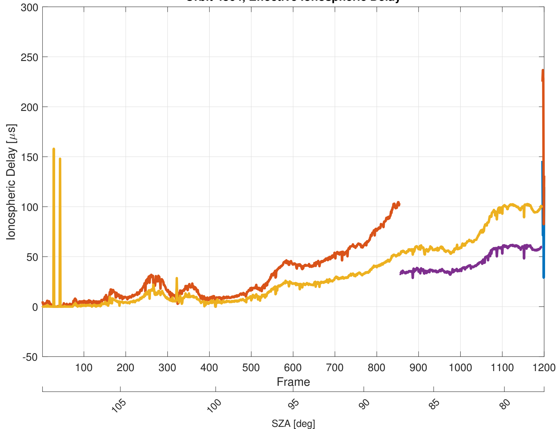
Orbit 4864, Effective Ionospheric Delay
