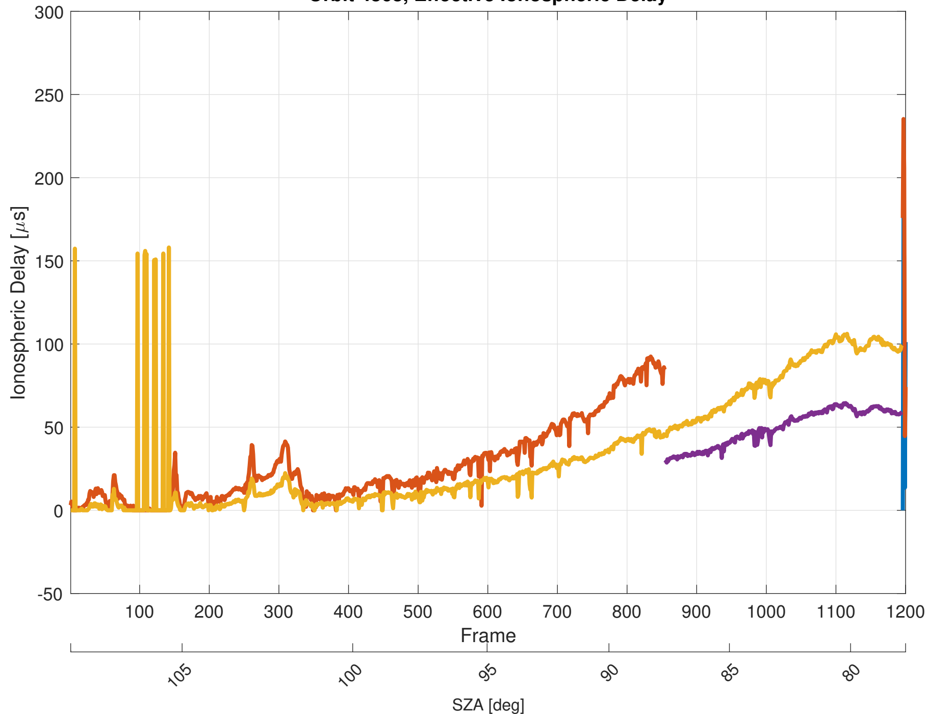
Orbit 4868, Effective Ionospheric Delay
