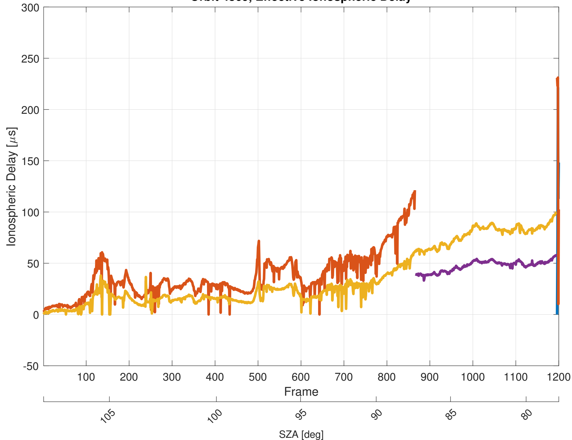
Orbit 4869, Effective Ionospheric Delay
