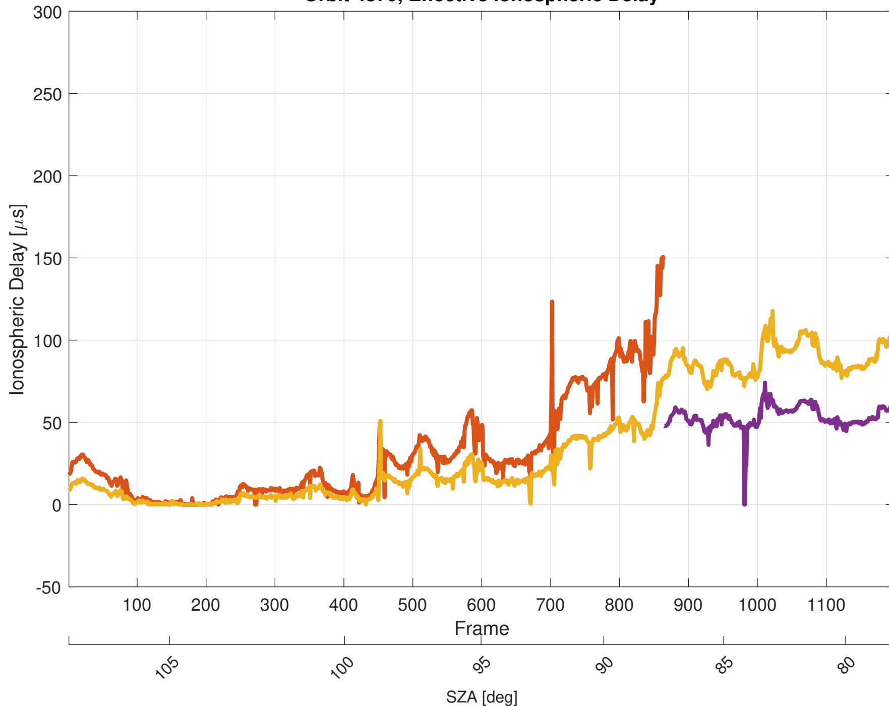
Orbit 4870, Effective Ionospheric Delay
