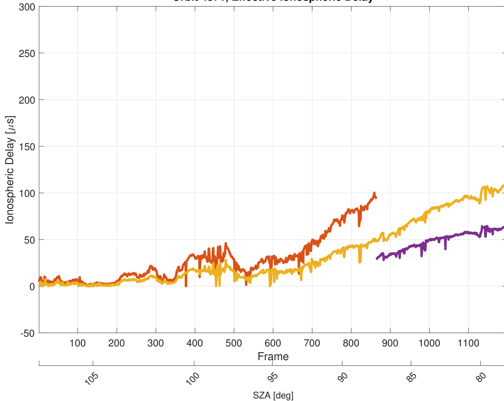
Orbit 4871, Effective Ionospheric Delay
