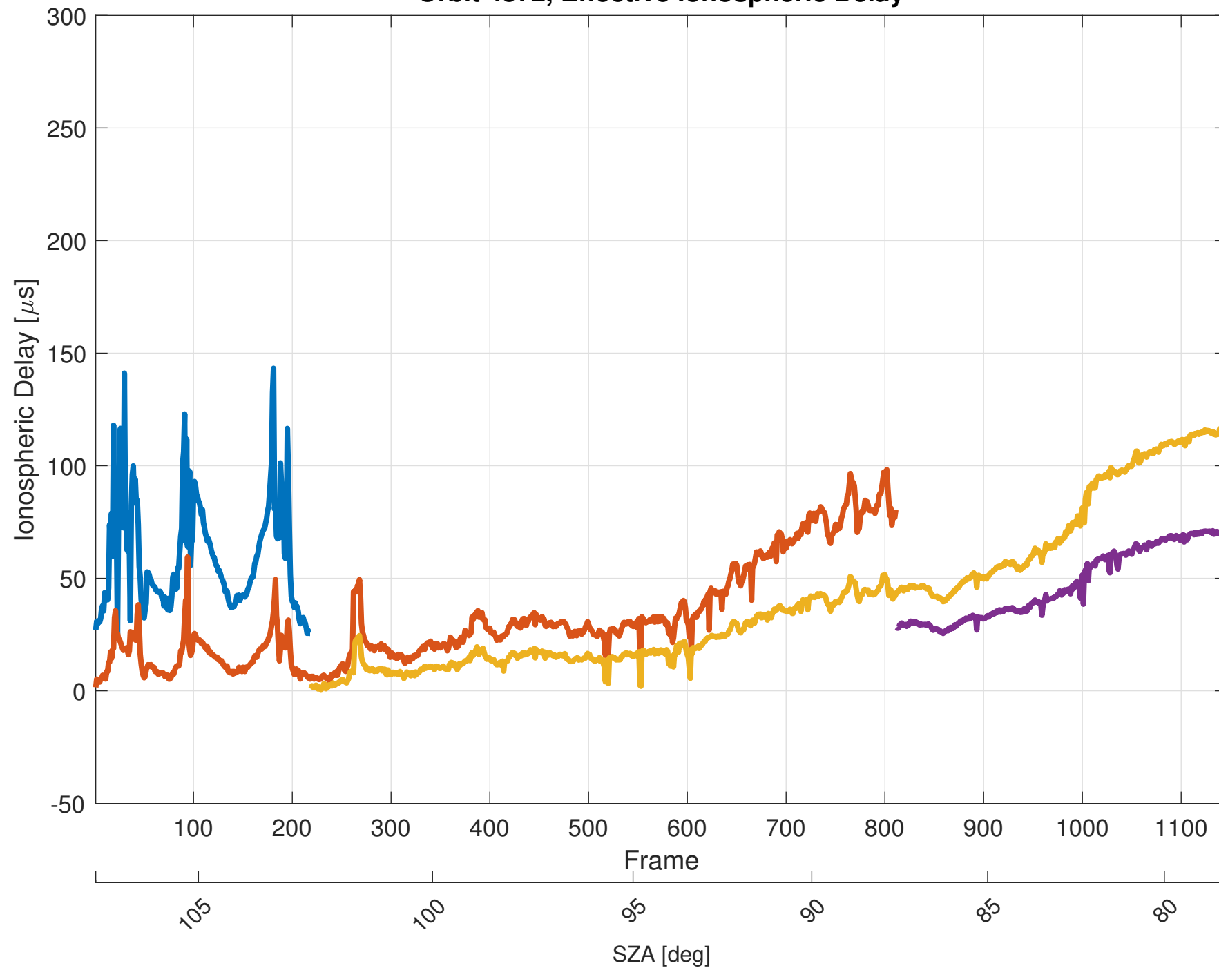
Orbit 4872, Effective Ionospheric Delay
