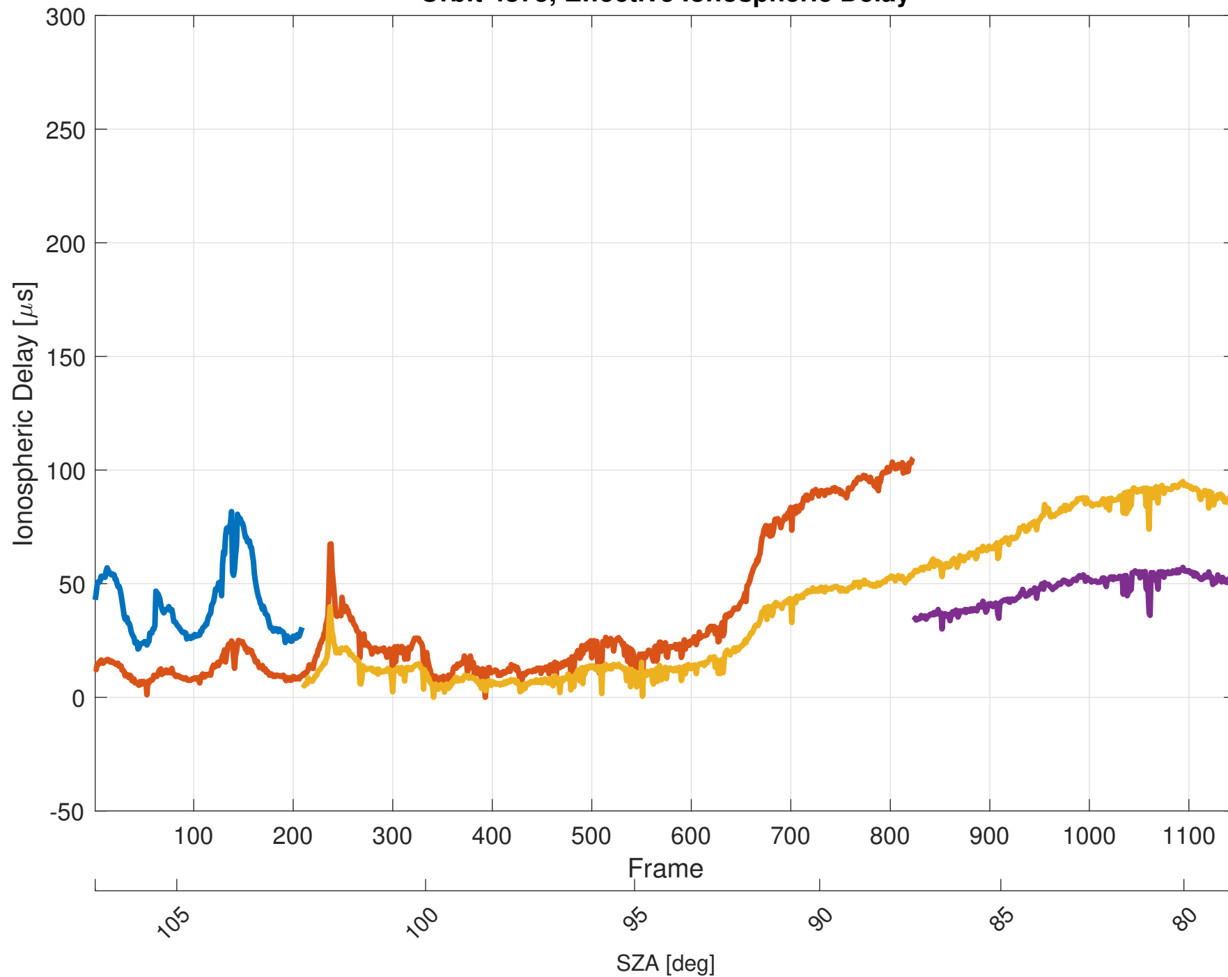
Orbit 4875, Effective Ionospheric Delay
