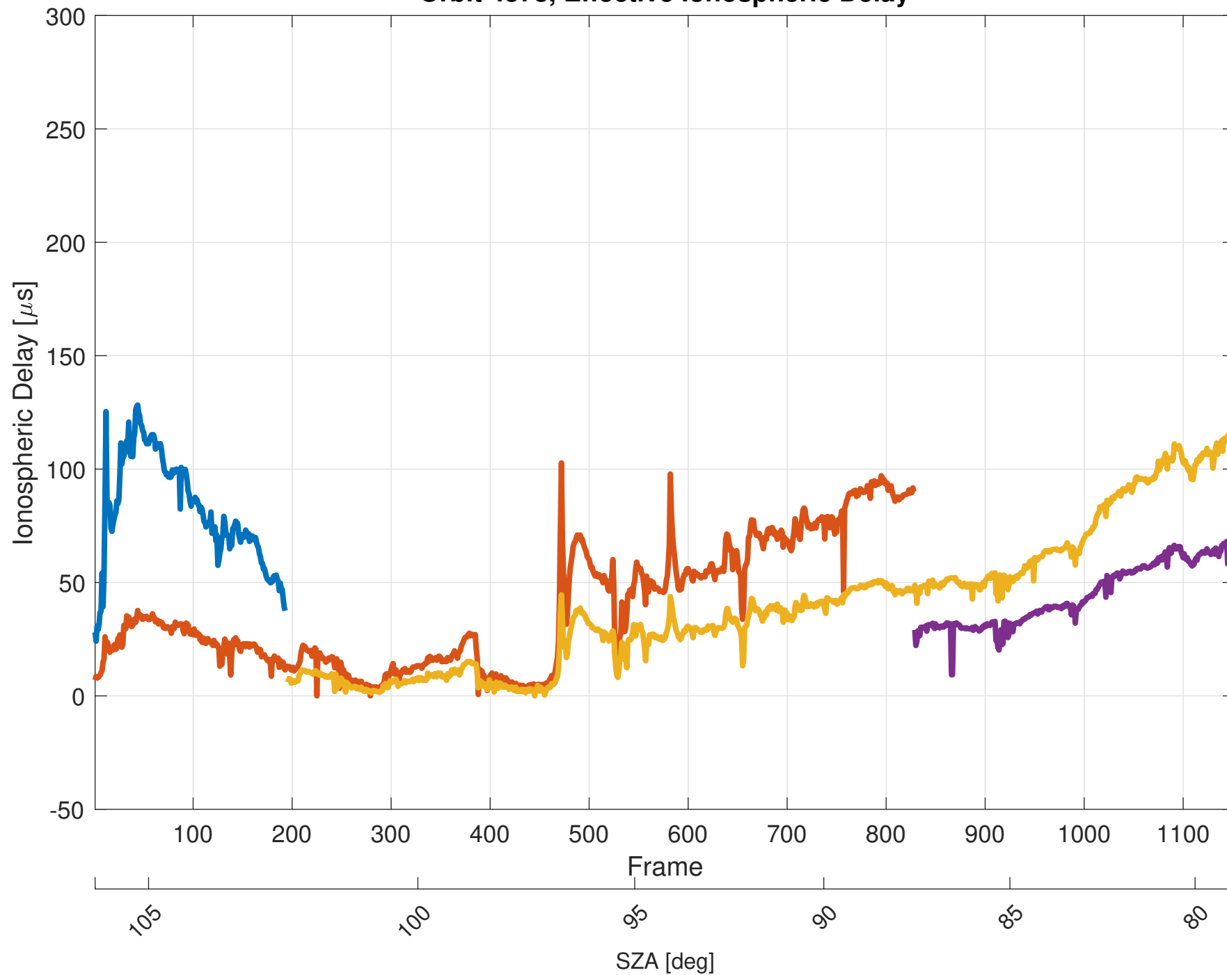
Orbit 4878, Effective Ionospheric Delay
