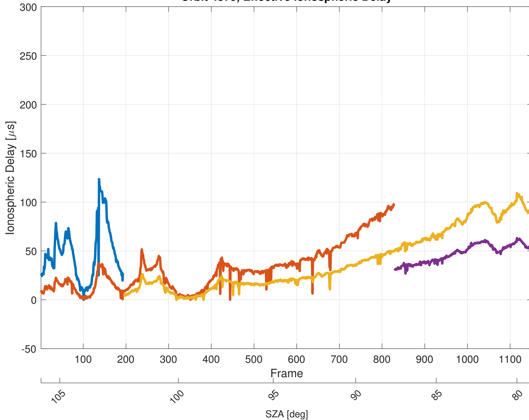
Orbit 4879, Effective Ionospheric Delay
