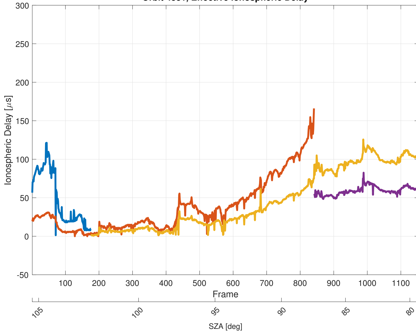
Orbit 4881, Effective Ionospheric Delay
