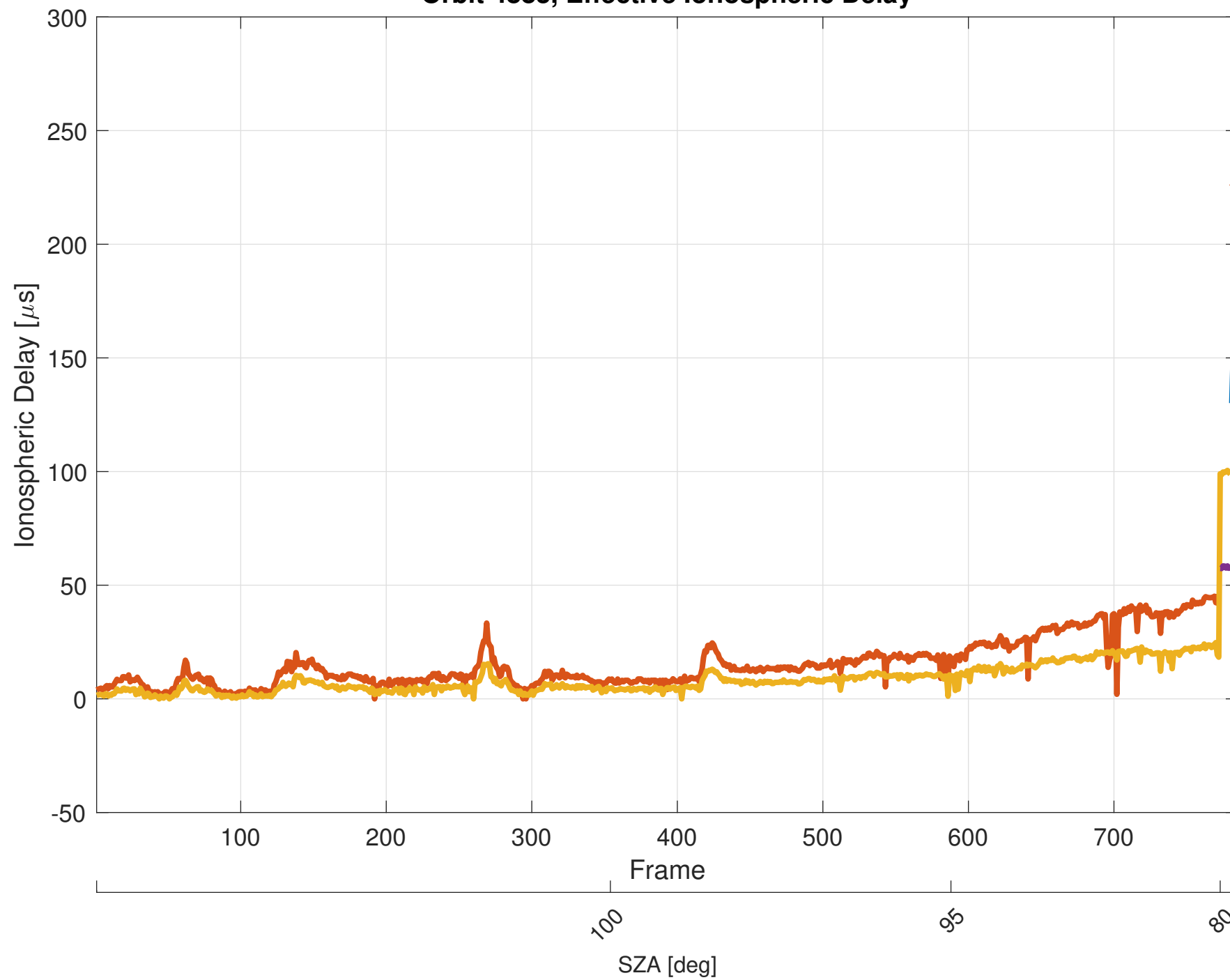
Orbit 4883, Effective Ionospheric Delay
