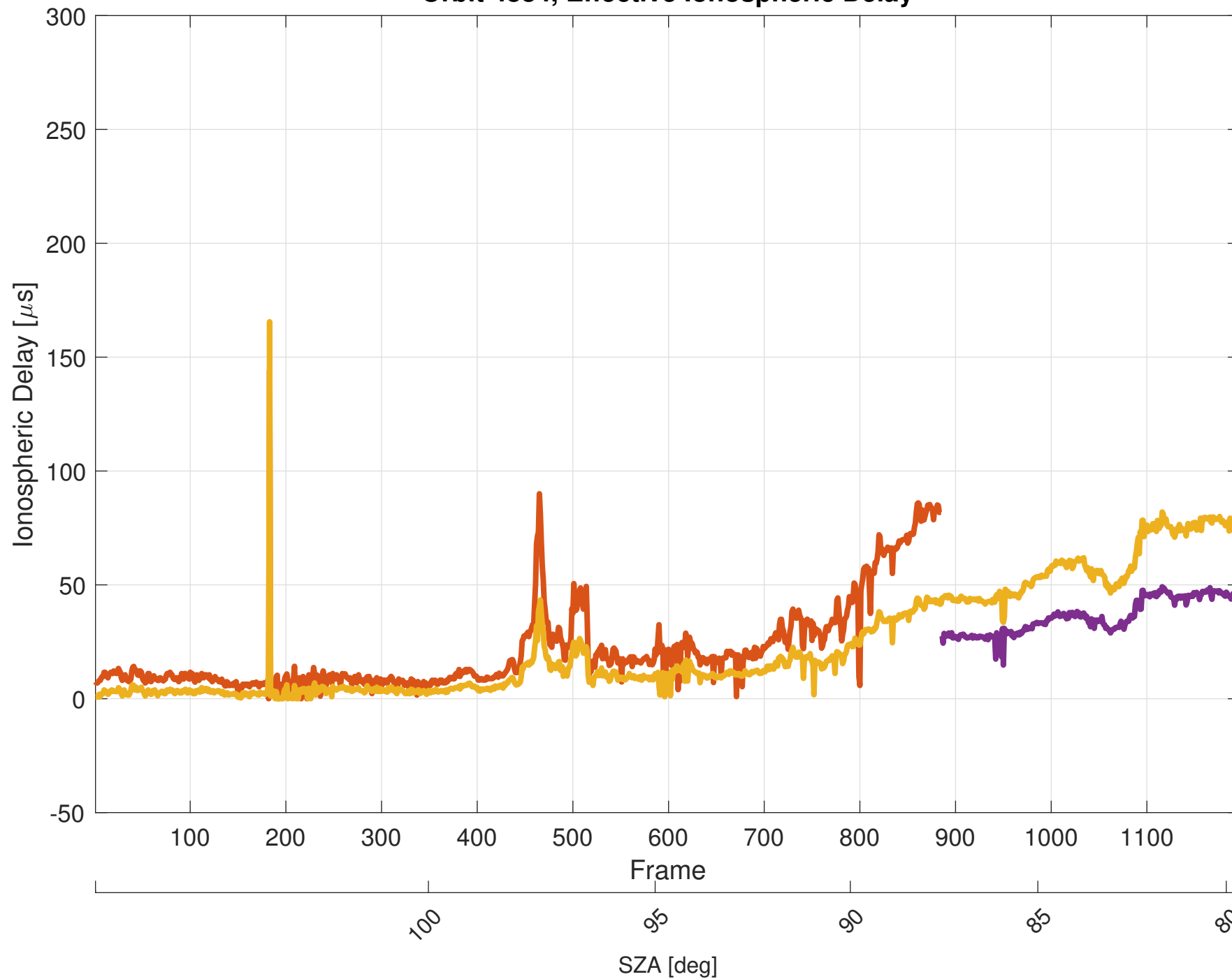
Orbit 4884, Effective Ionospheric Delay
