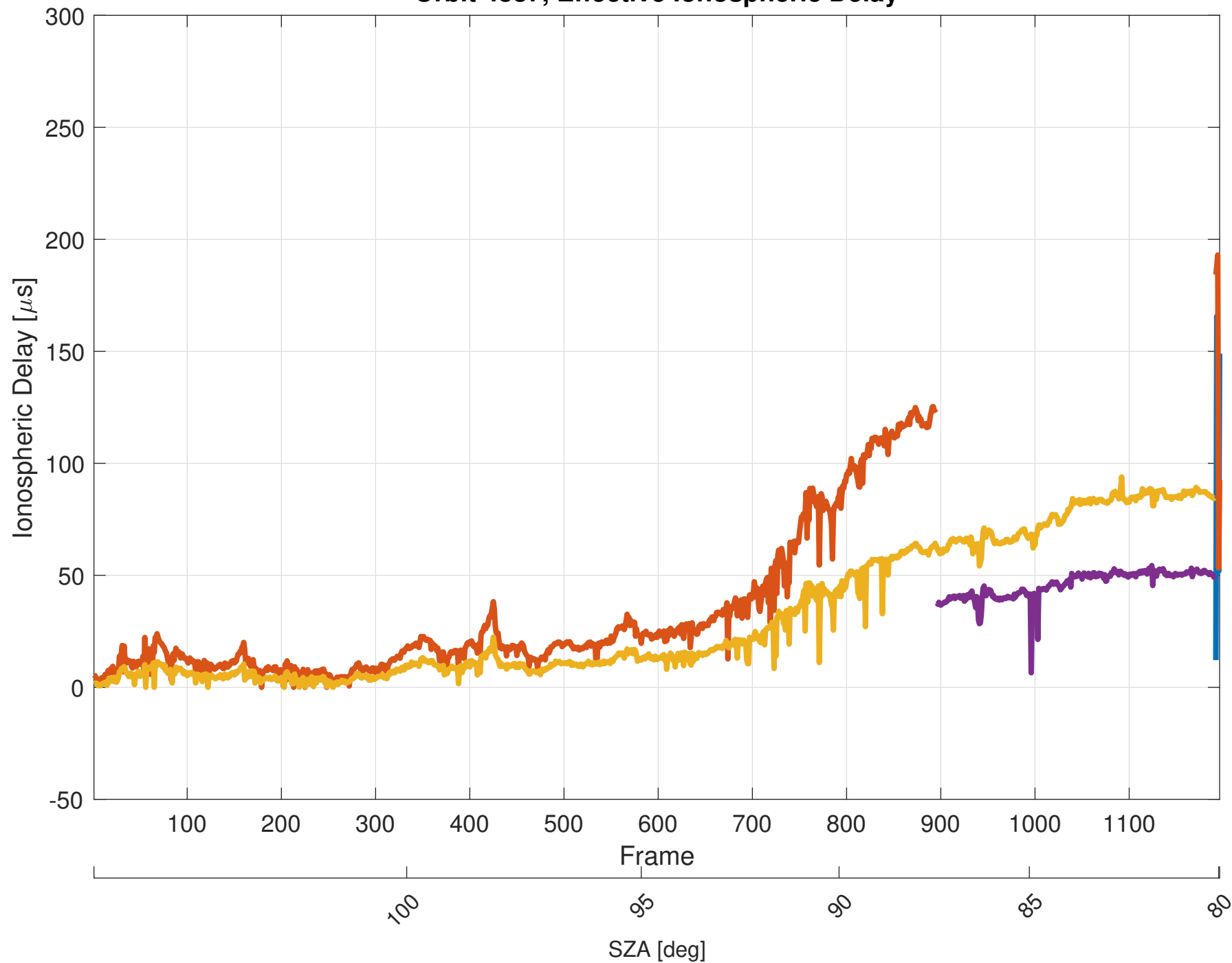
Orbit 4887, Effective Ionospheric Delay
