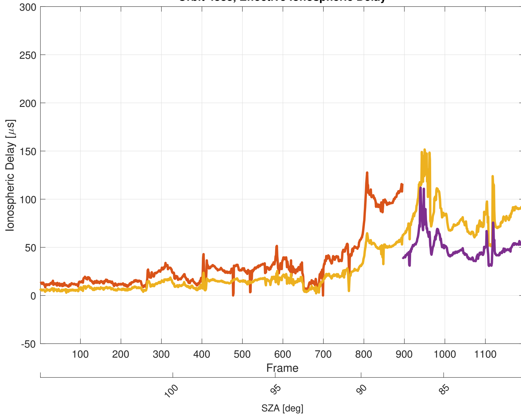
Orbit 4888, Effective Ionospheric Delay
