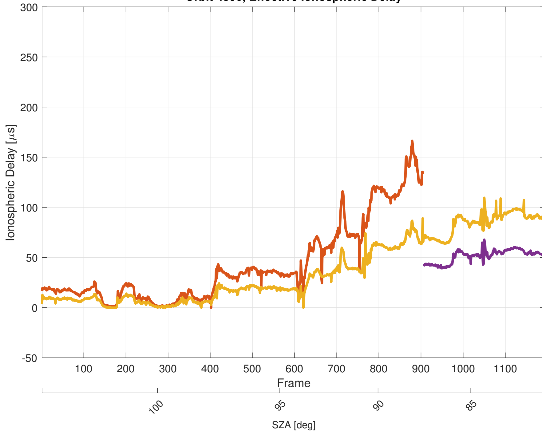
Orbit 4896, Effective Ionospheric Delay
