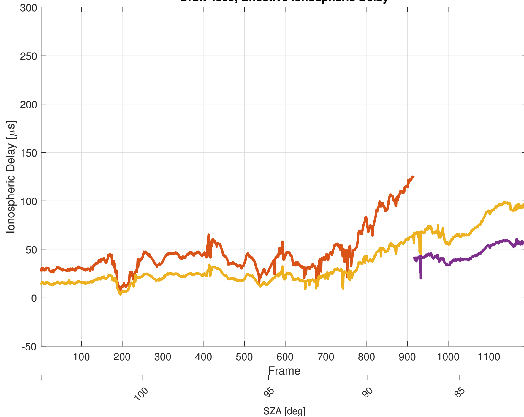
Orbit 4899, Effective Ionospheric Delay
