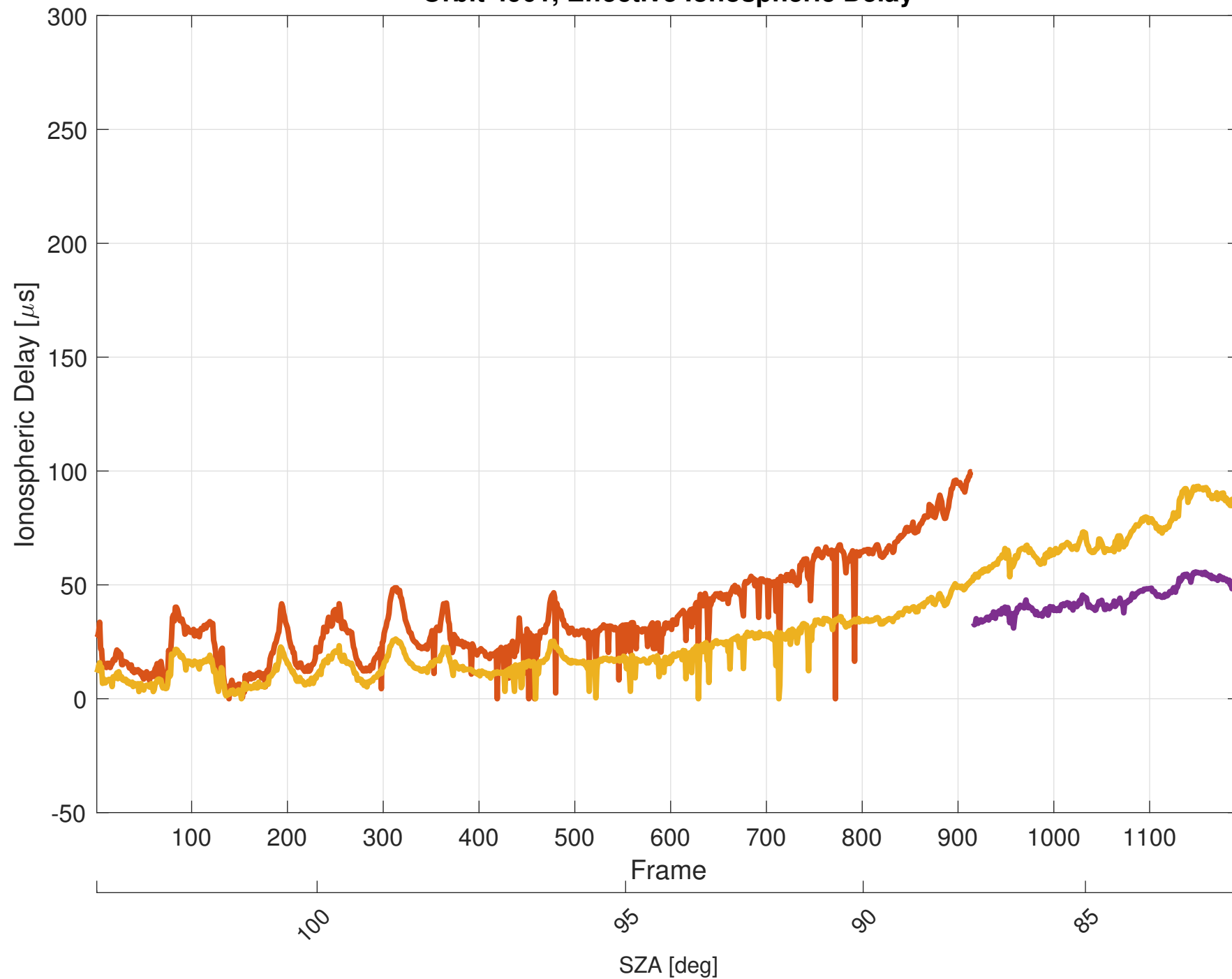
Orbit 4901, Effective Ionospheric Delay
