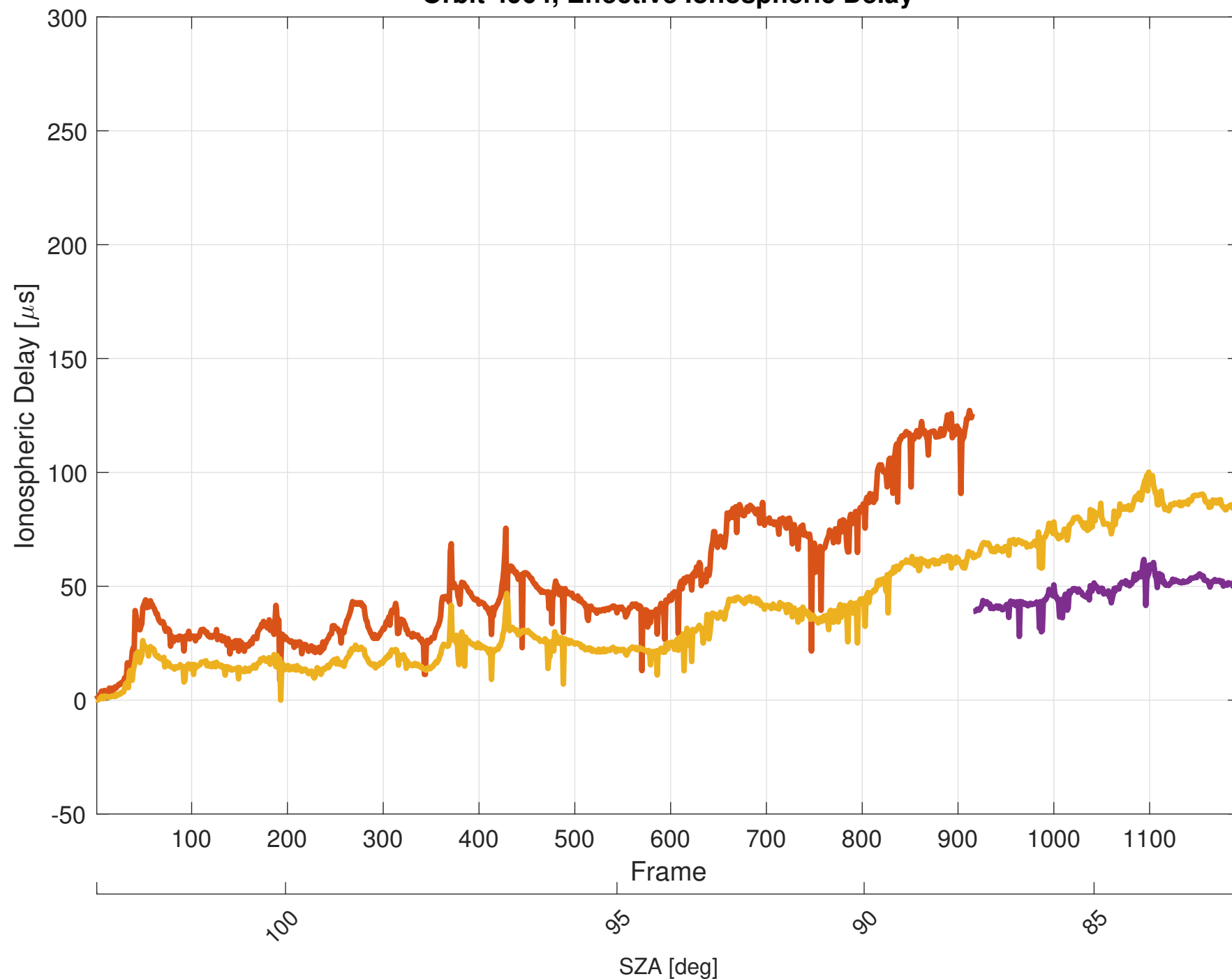
Orbit 4904, Effective Ionospheric Delay
