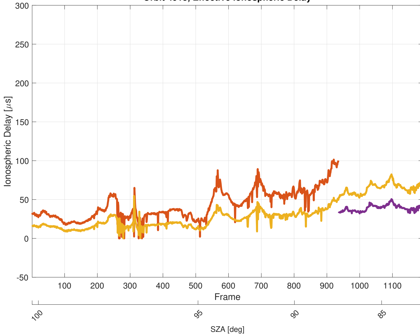
Orbit 4913, Effective Ionospheric Delay
