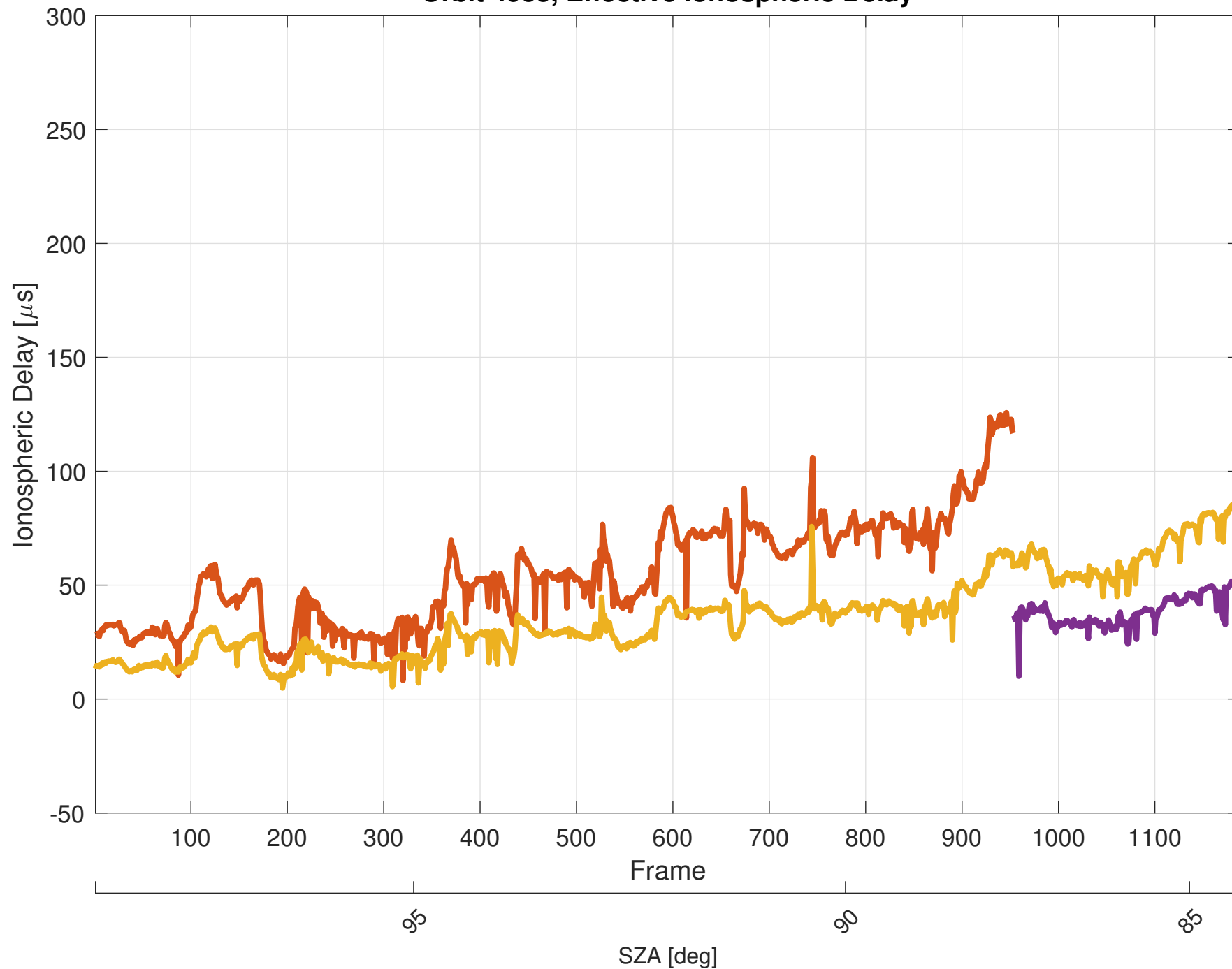
Orbit 4933, Effective Ionospheric Delay
