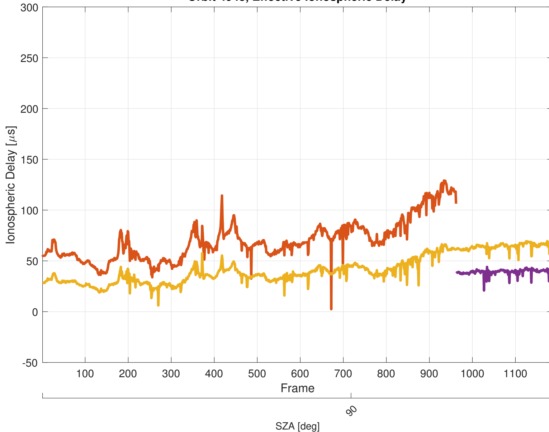
Orbit 4948, Effective Ionospheric Delay
