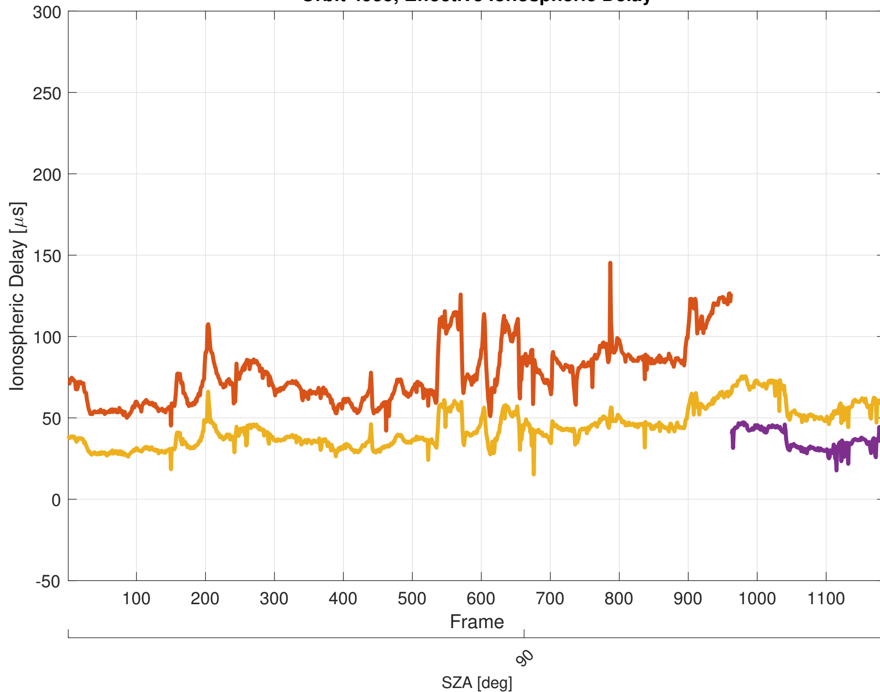
Orbit 4955, Effective Ionospheric Delay
