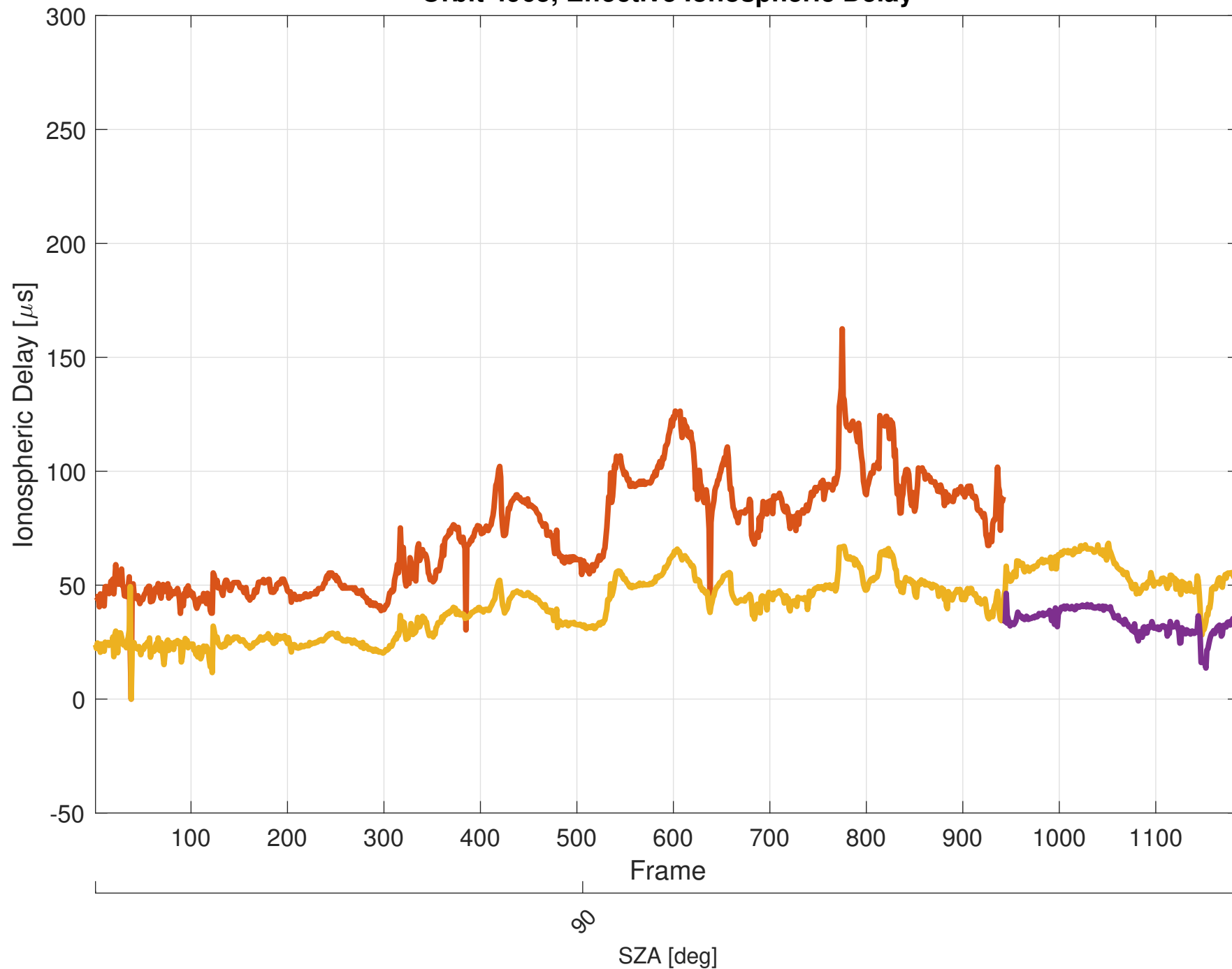
Orbit 4965, Effective Ionospheric Delay
