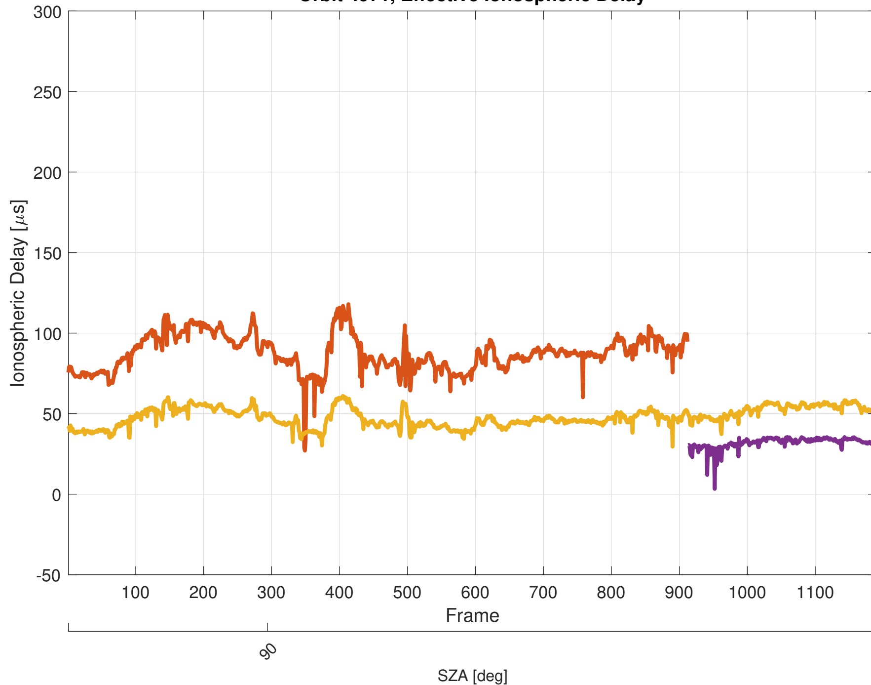
Orbit 4971, Effective Ionospheric Delay
