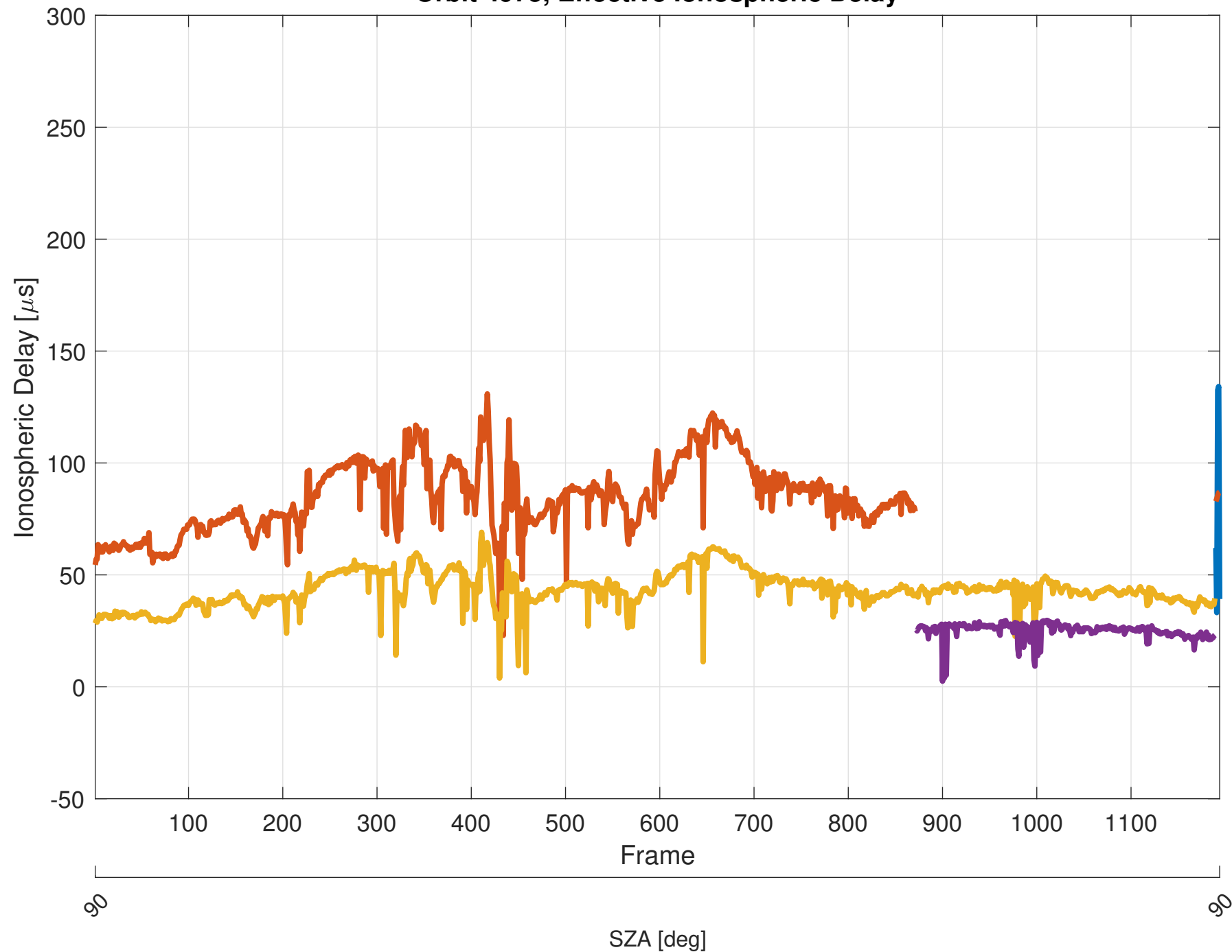
Orbit 4975, Effective Ionospheric Delay
