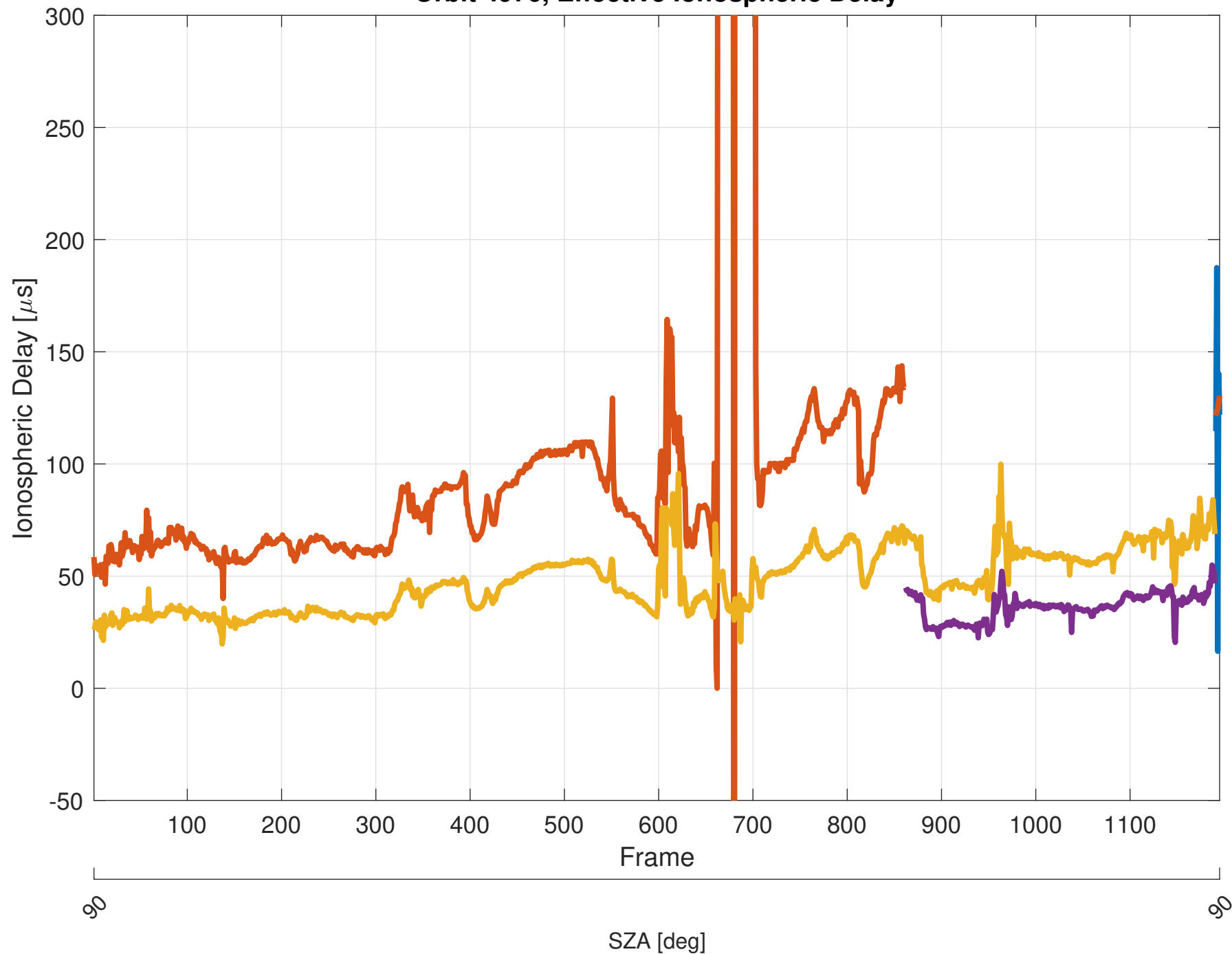
Orbit 4976, Effective Ionospheric Delay
