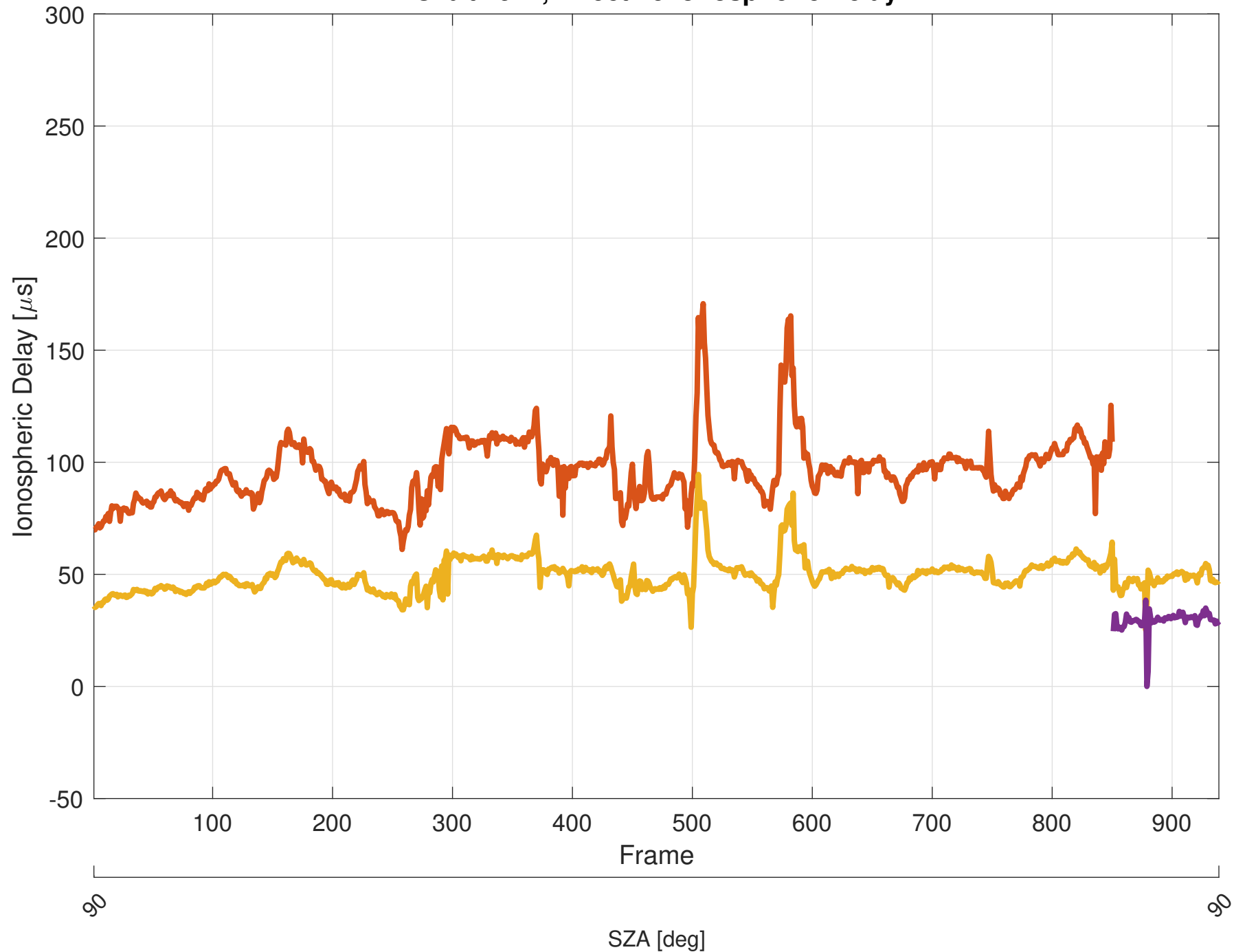
Orbit 4977, Effective Ionospheric Delay
