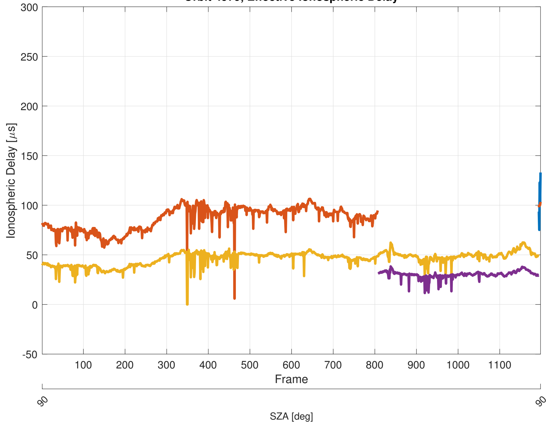
Orbit 4979, Effective Ionospheric Delay
