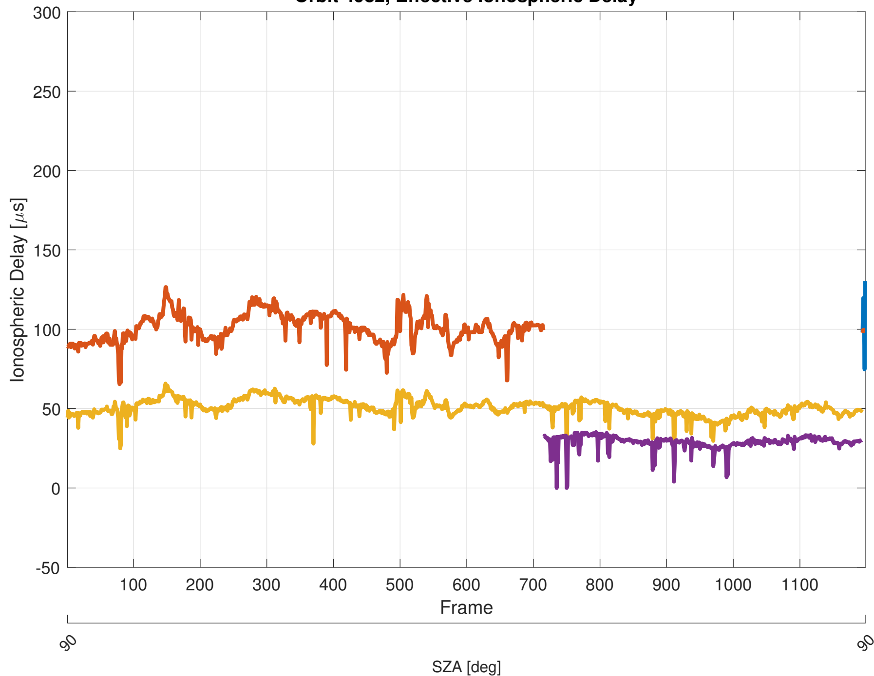
Orbit 4982, Effective Ionospheric Delay
