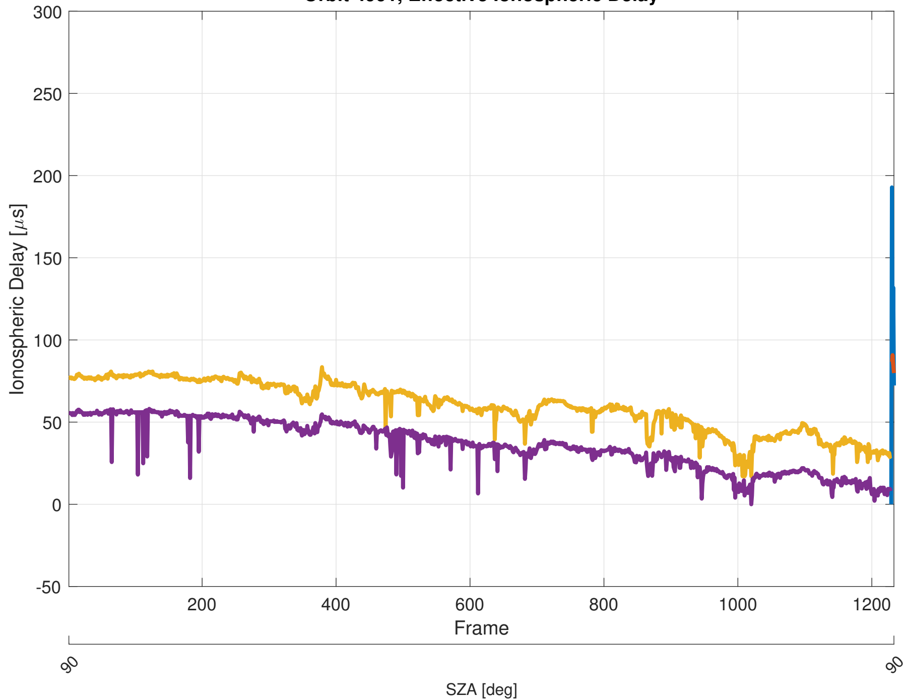
Orbit 4991, Effective Ionospheric Delay
