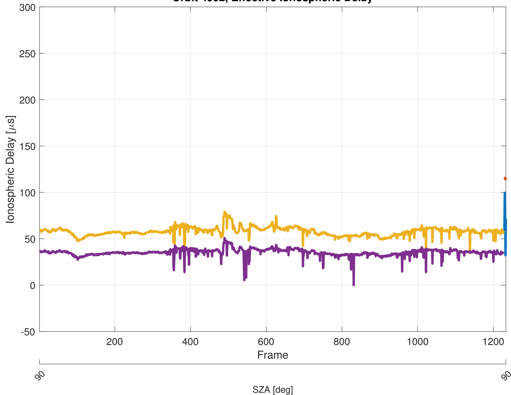
Orbit 4992, Effective Ionospheric Delay
