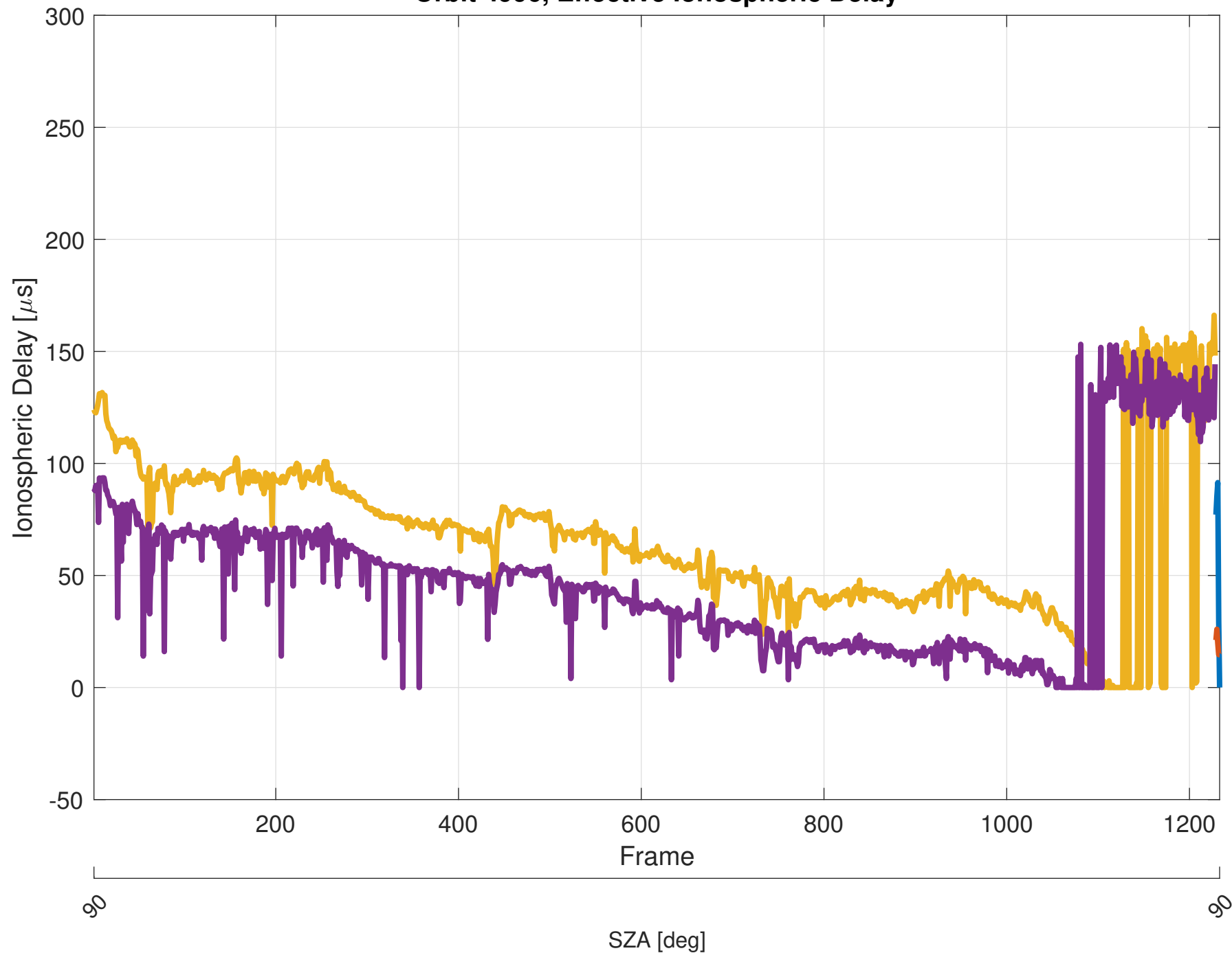
Orbit 4996, Effective Ionospheric Delay
