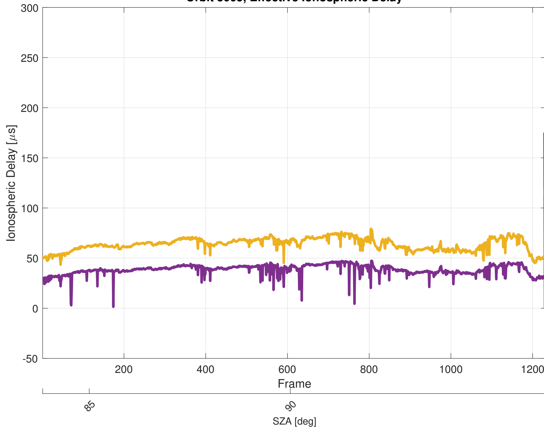
Orbit 5005, Effective Ionospheric Delay
