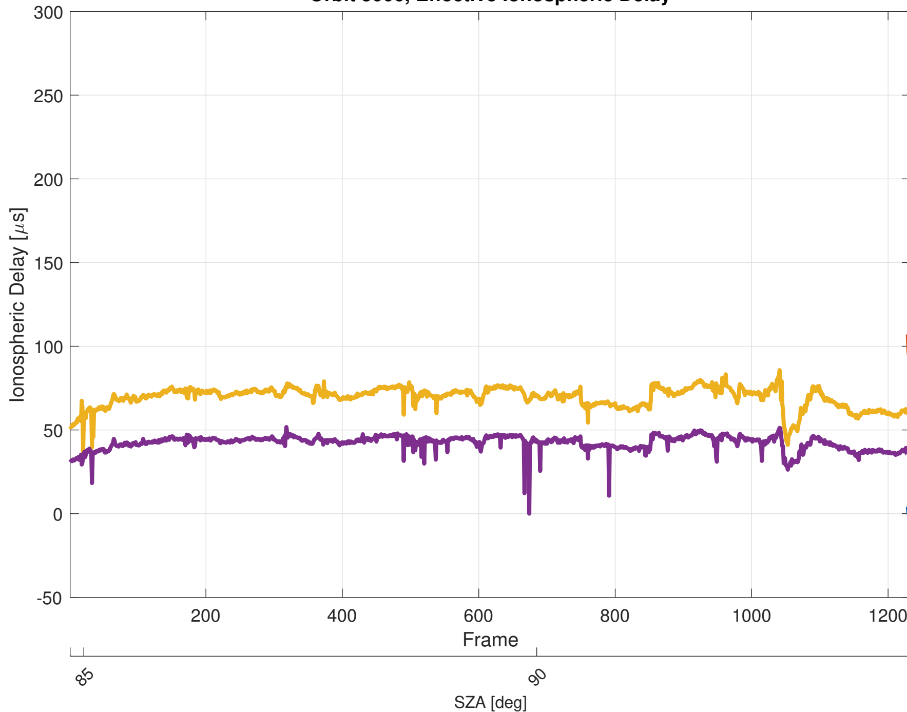
Orbit 5006, Effective Ionospheric Delay
