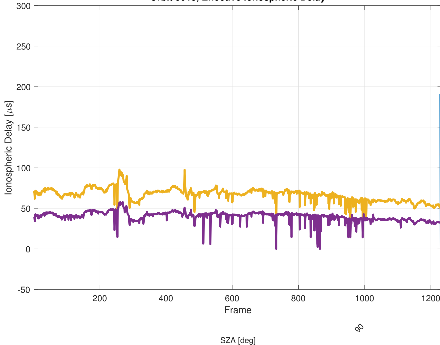
Orbit 5018, Effective Ionospheric Delay
