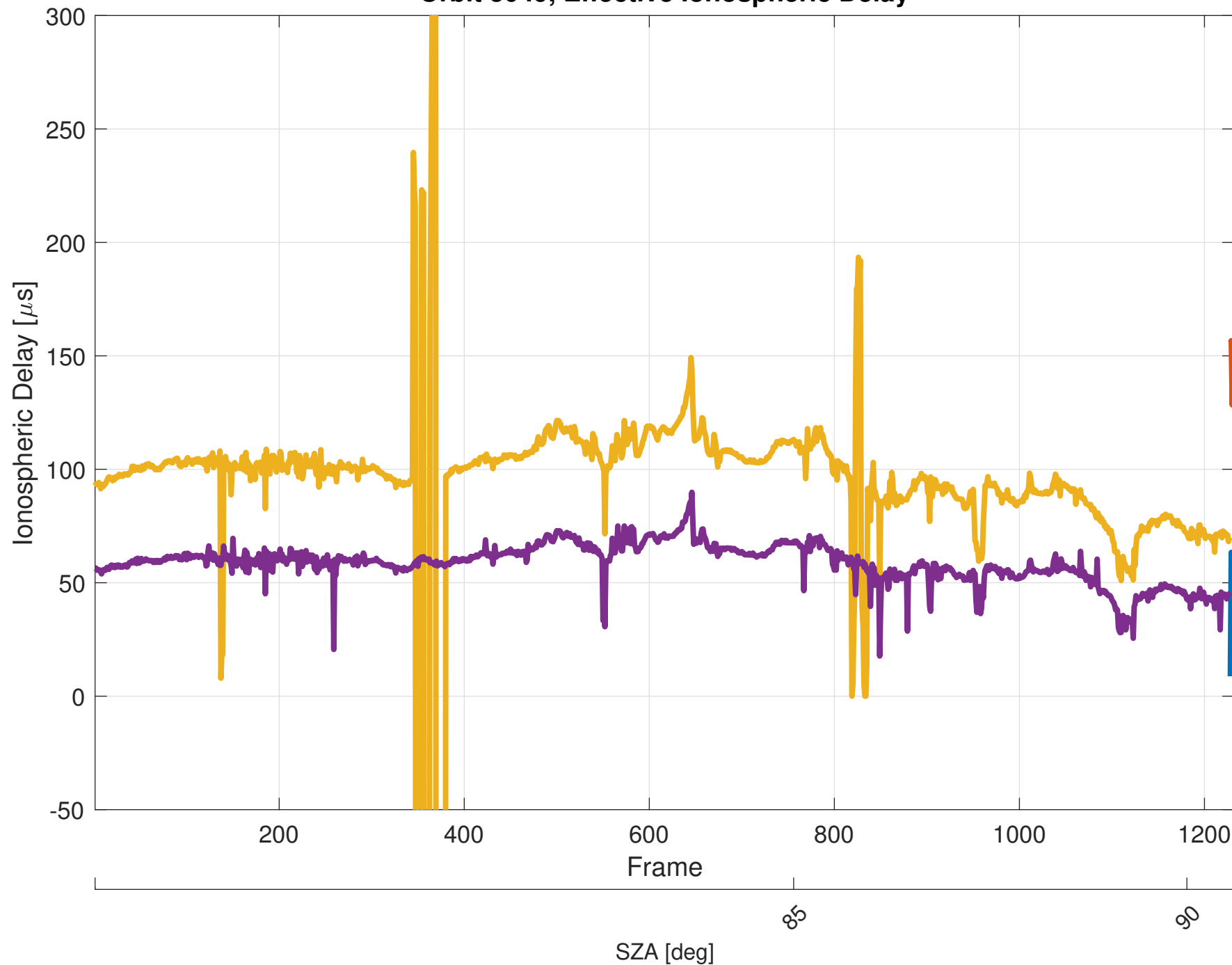
Orbit 5049, Effective Ionospheric Delay
