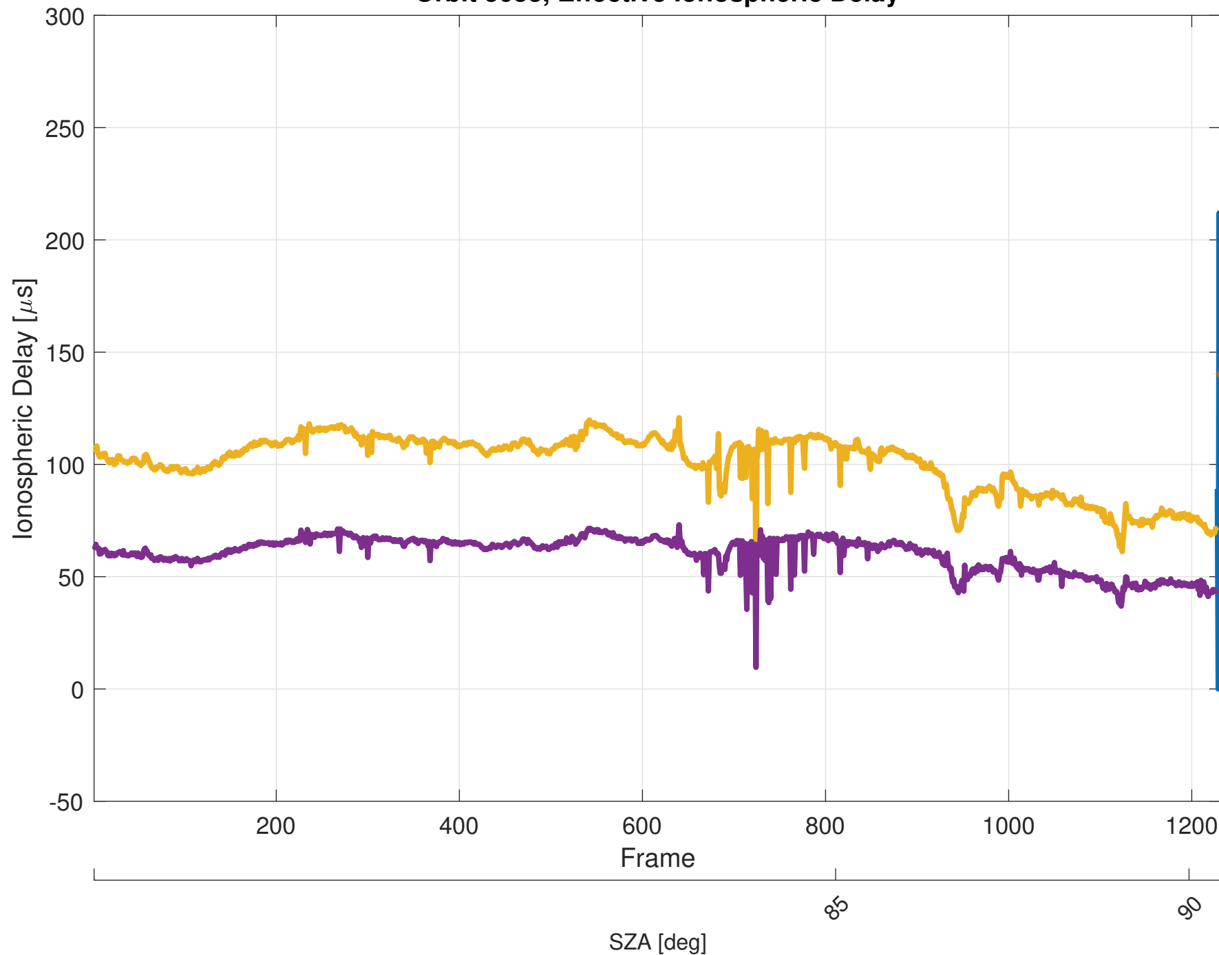
Orbit 5053, Effective Ionospheric Delay
