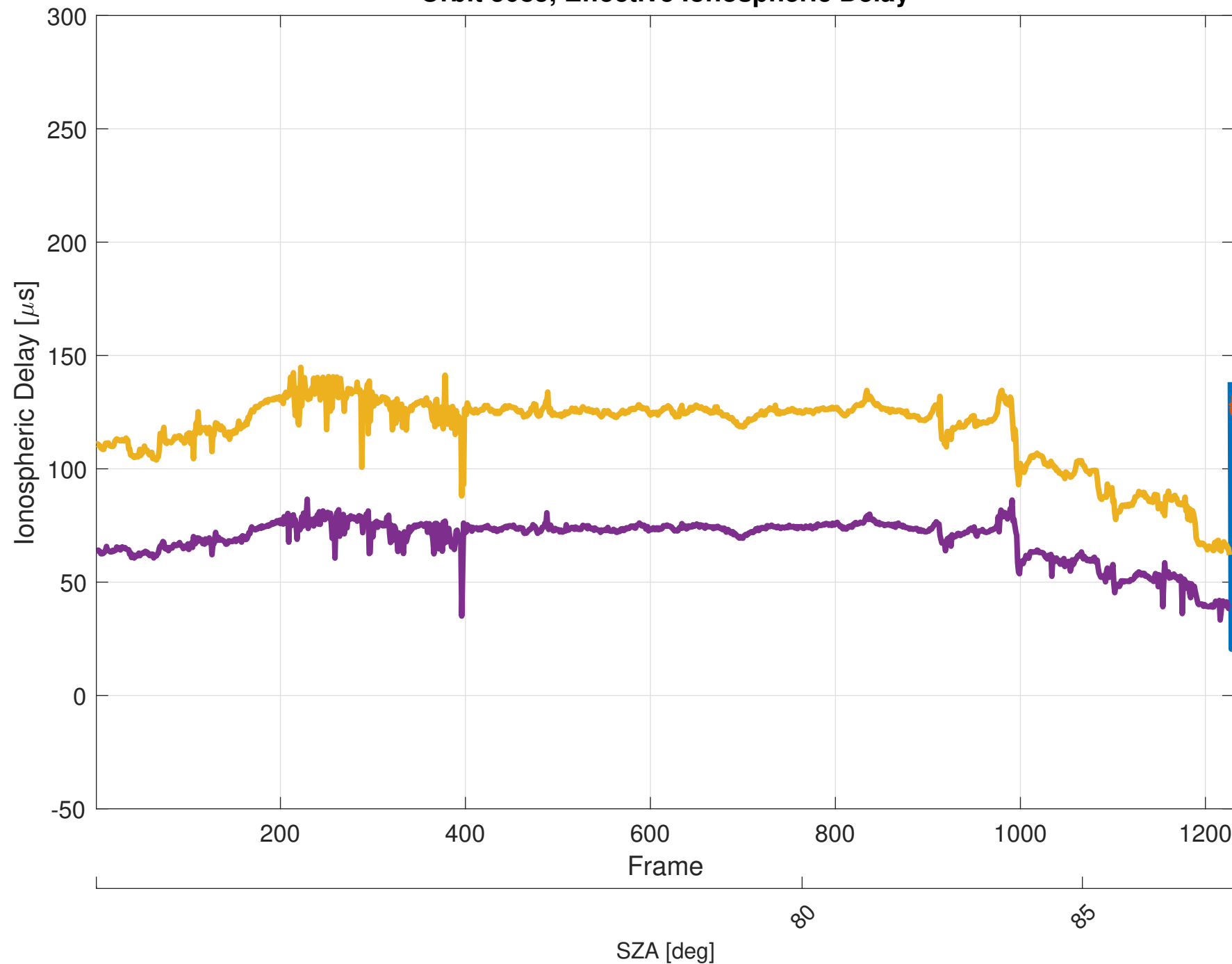
Orbit 5085, Effective Ionospheric Delay
