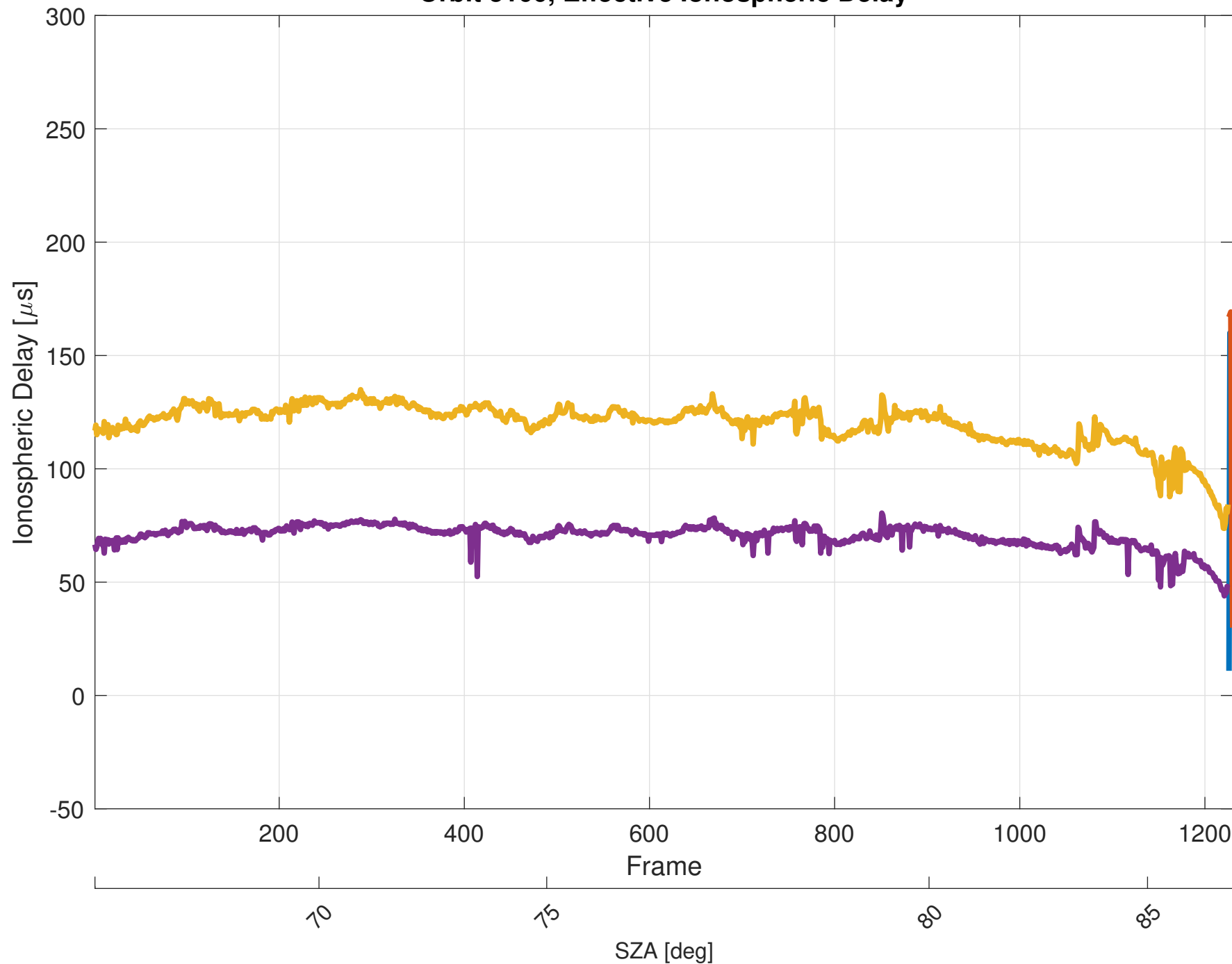
Orbit 5100, Effective Ionospheric Delay
