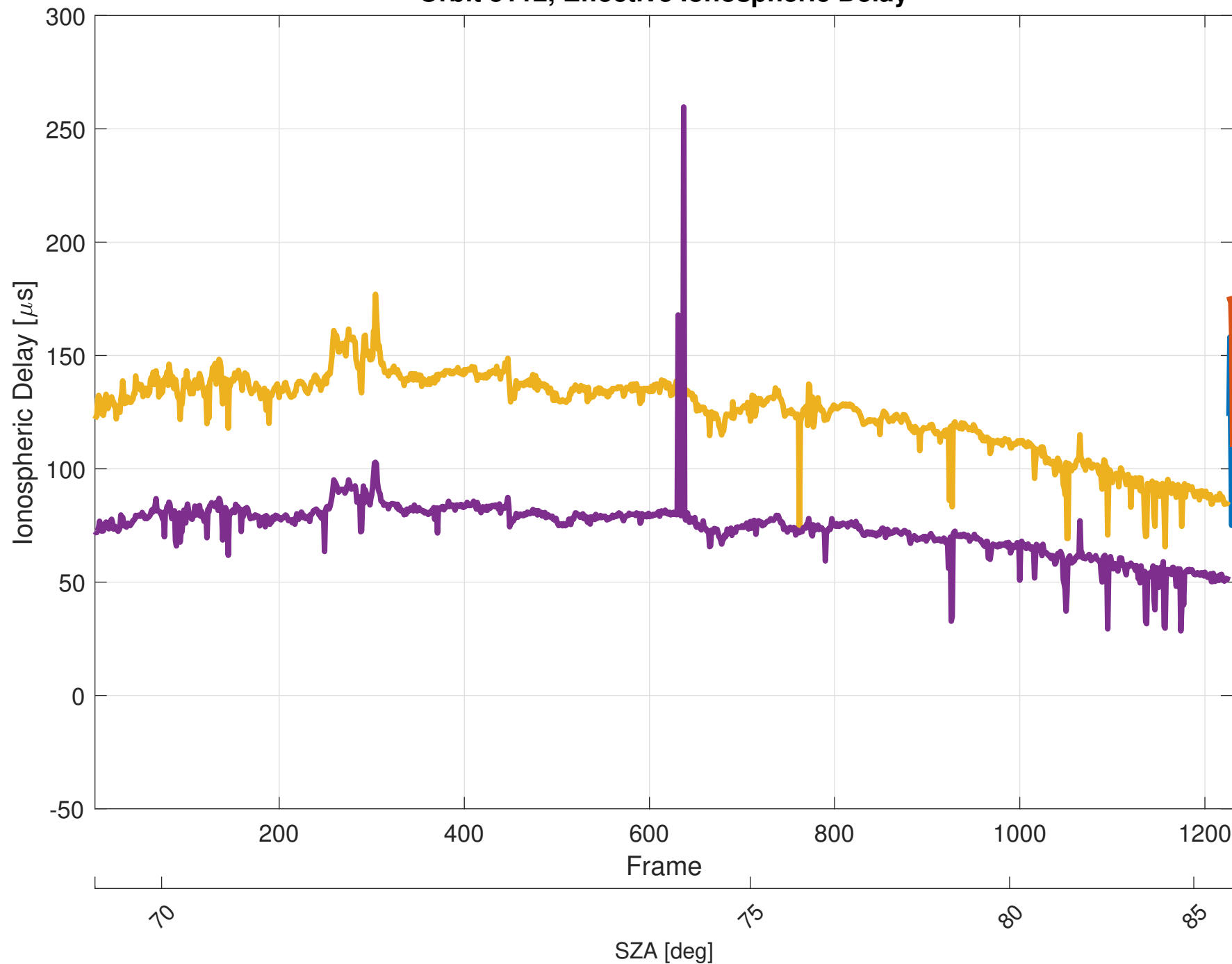
Orbit 5112, Effective Ionospheric Delay
