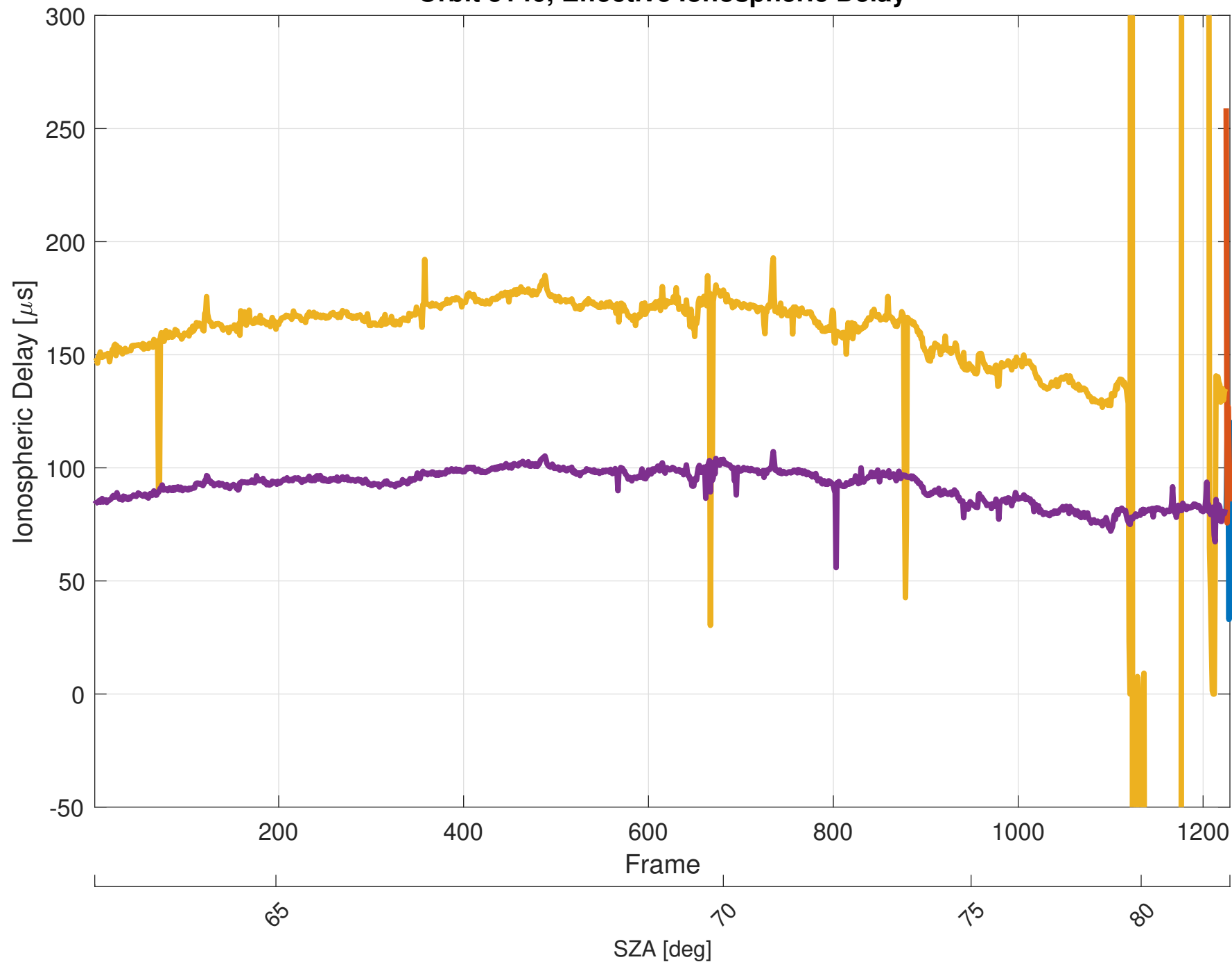
Orbit 5140, Effective Ionospheric Delay
