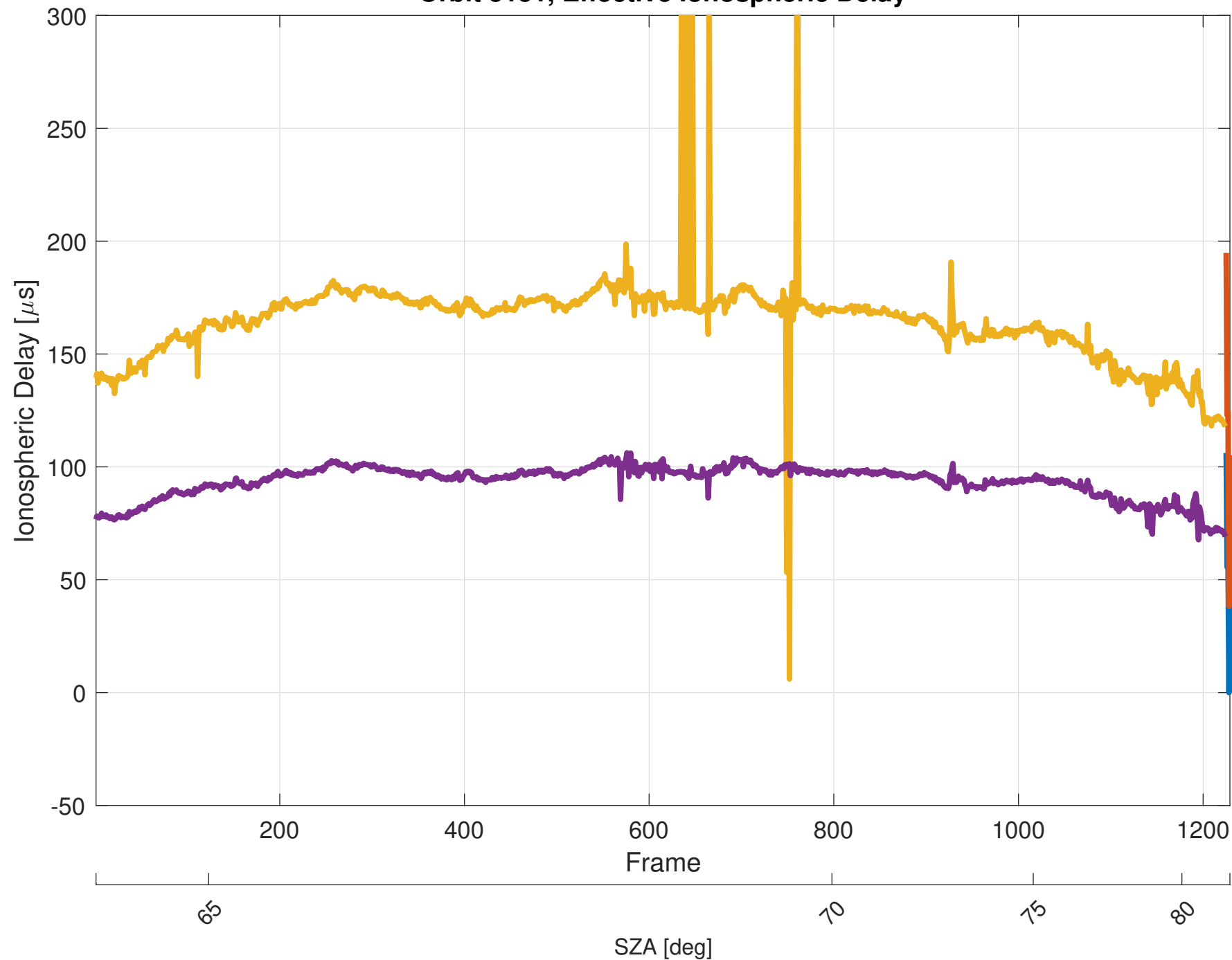
Orbit 5151, Effective Ionospheric Delay
