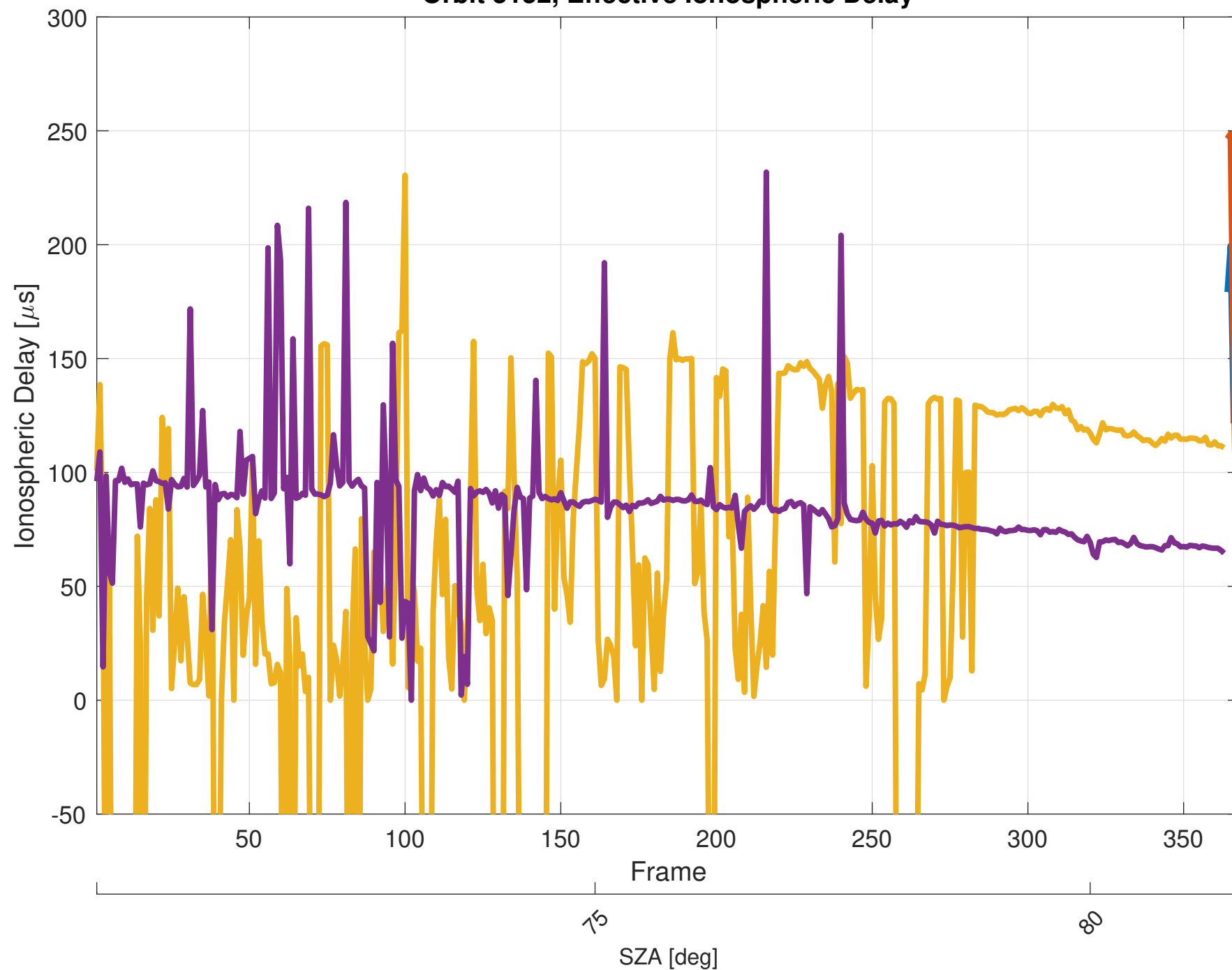
Orbit 5152, Effective Ionospheric Delay
