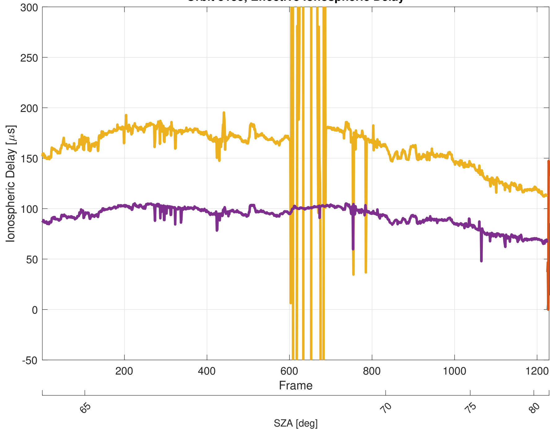
Orbit 5155, Effective Ionospheric Delay
