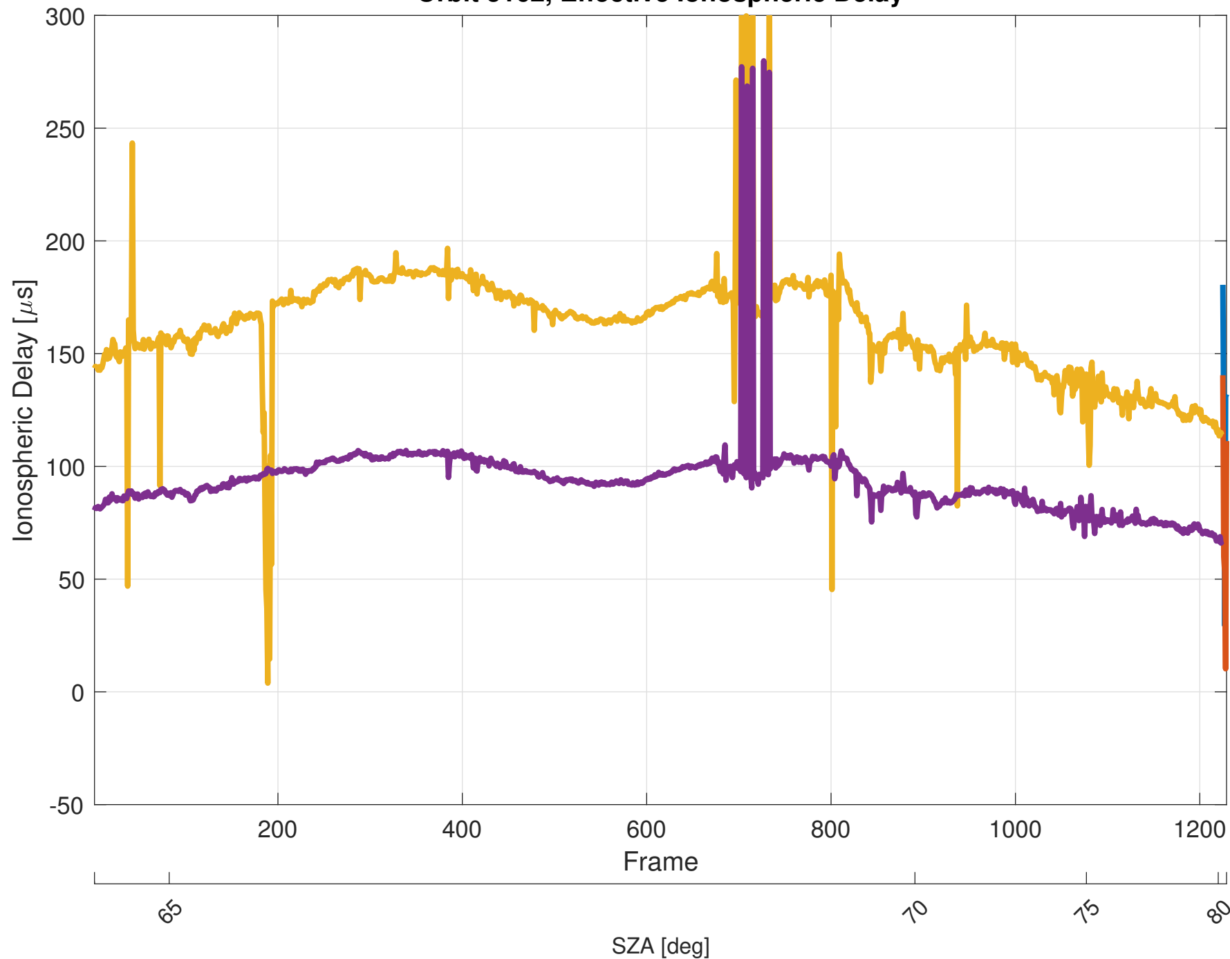
Orbit 5162, Effective Ionospheric Delay
