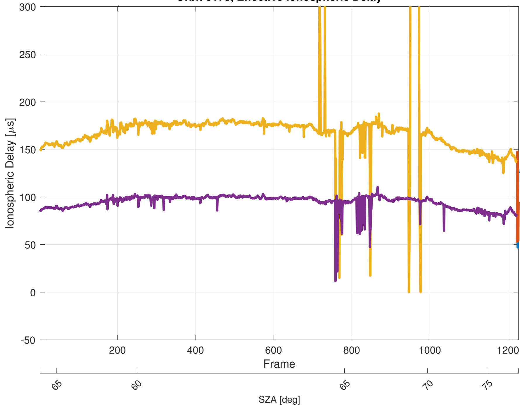
Orbit 5178, Effective Ionospheric Delay
