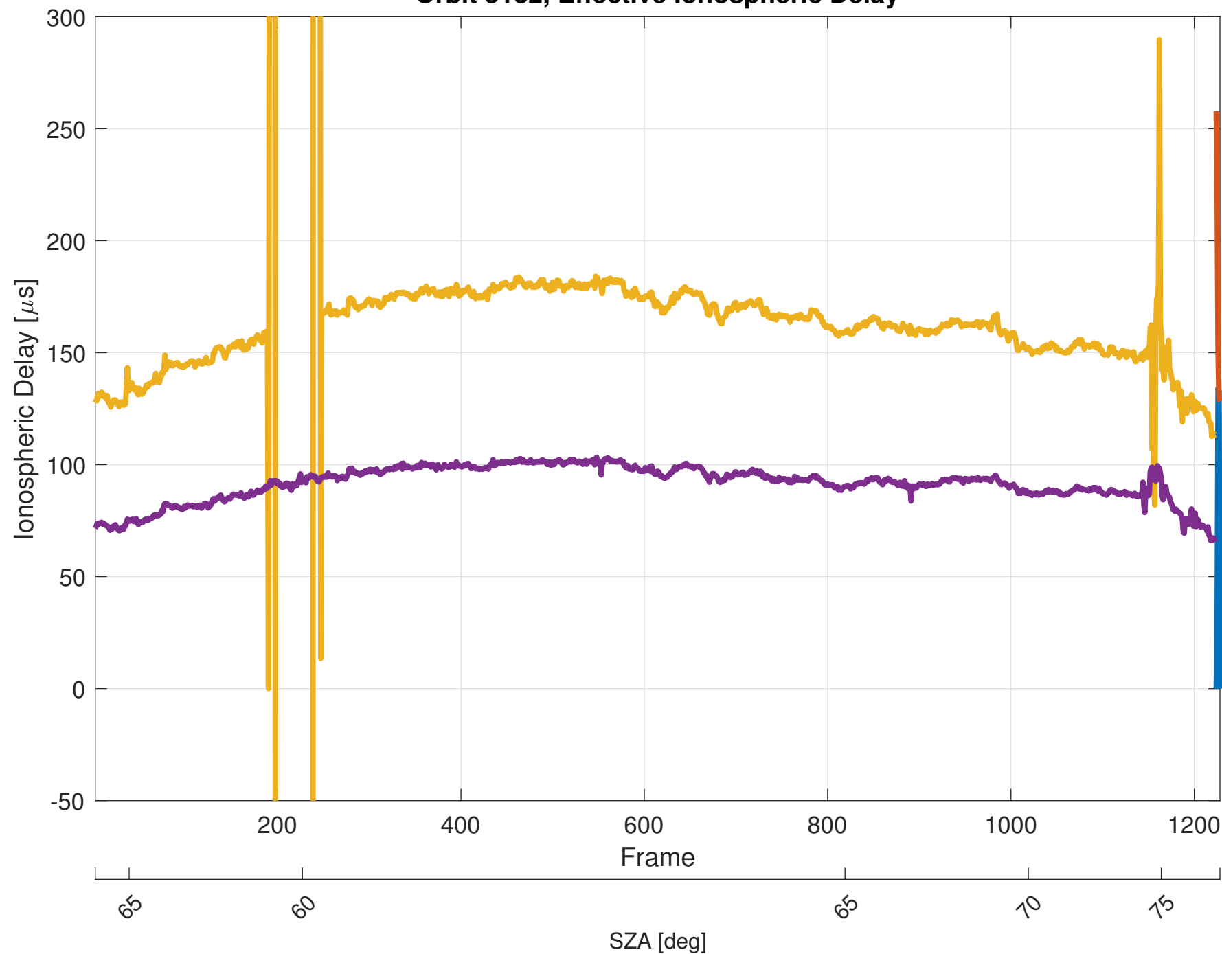
Orbit 5182, Effective Ionospheric Delay
