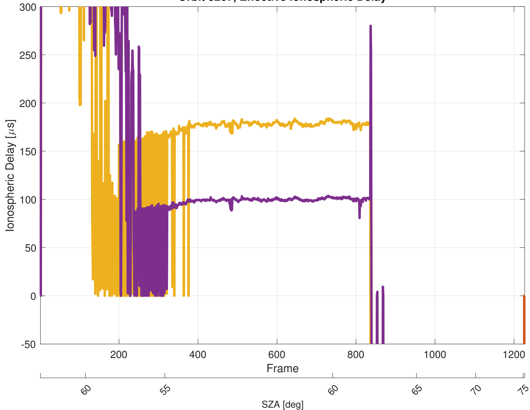
Orbit 5207, Effective Ionospheric Delay
