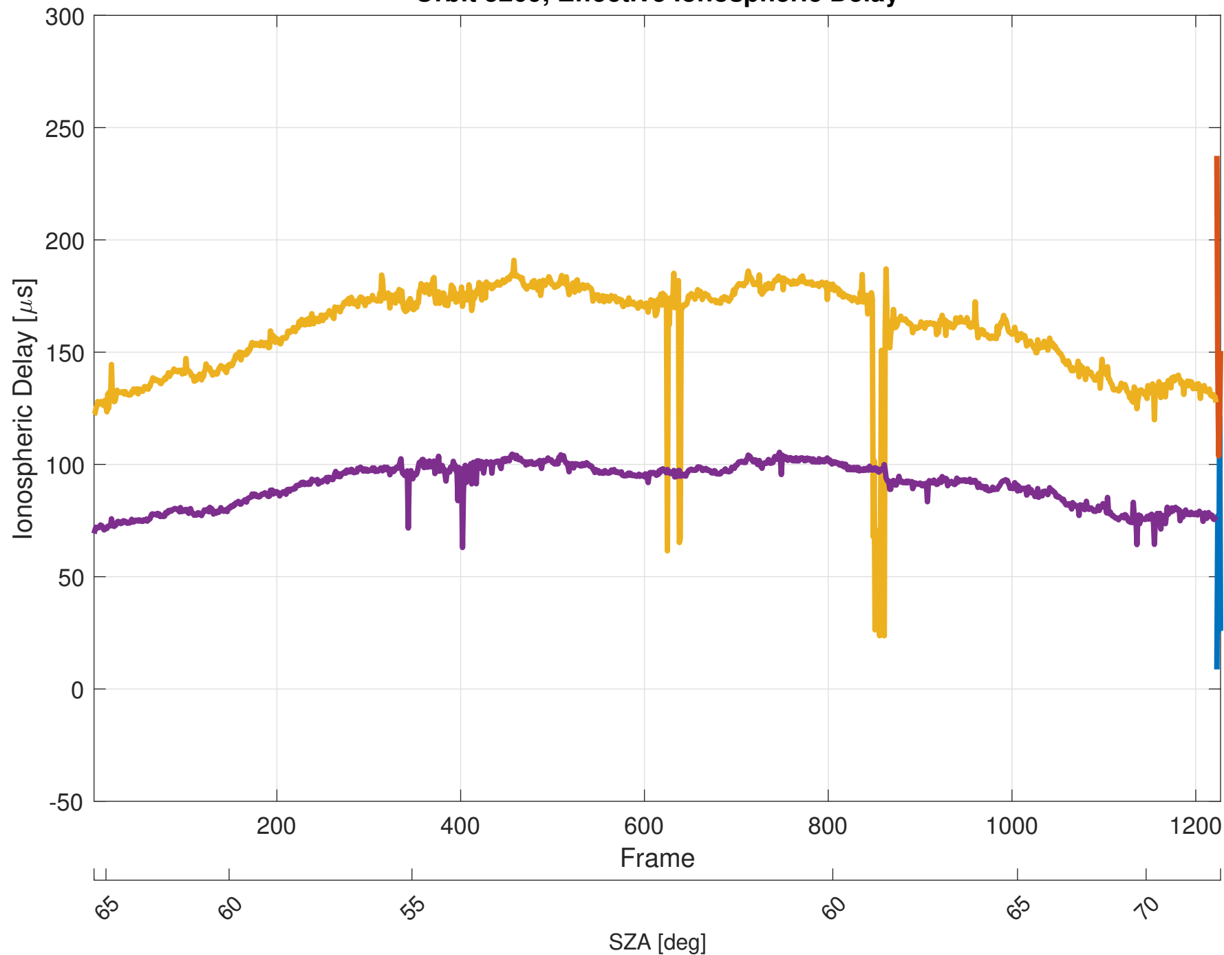
Orbit 5209, Effective Ionospheric Delay
