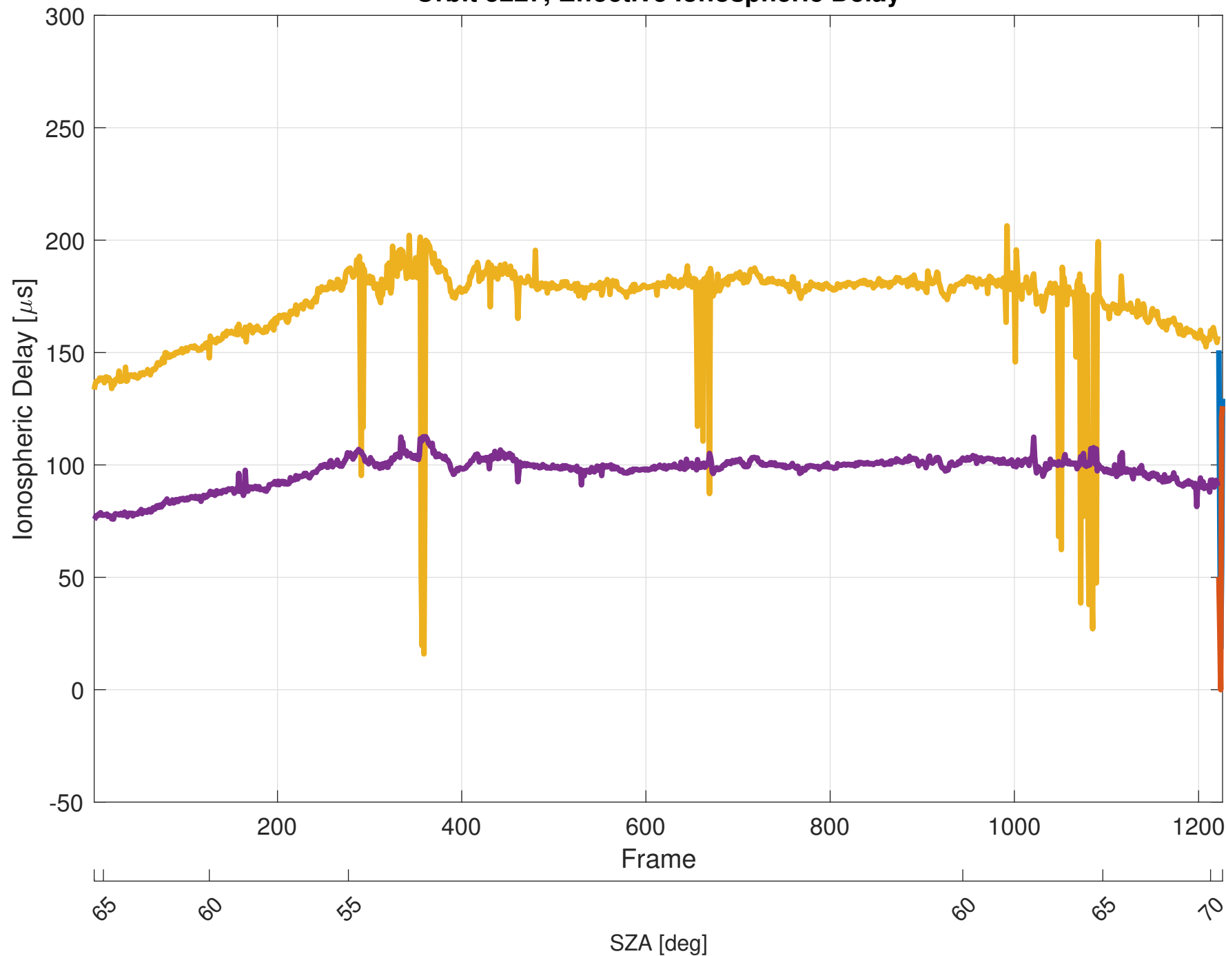
Orbit 5227, Effective Ionospheric Delay
